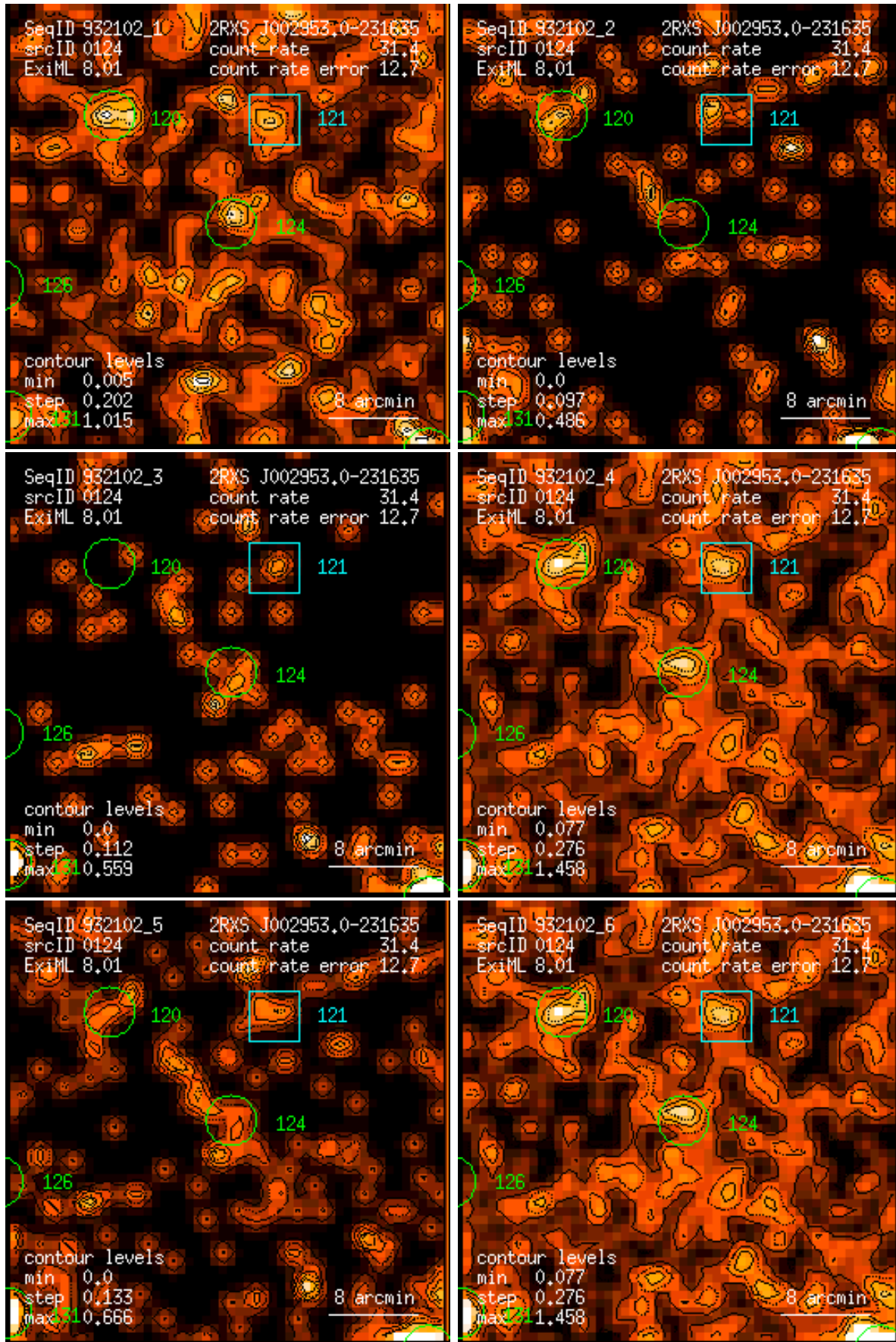
Figure 124: RASS 932102: detection 0124: band rate images, Gaussian filter: (1) PSPC channels 11 – 41, (2) 52 – 90, (3) 91 – 201, (4) 11 – 235, (5) 52 – 201, (6) 11 – 201. Broad band rates in counts/ks. Band rate contour levels in counts/ks/arcmin 2 .
