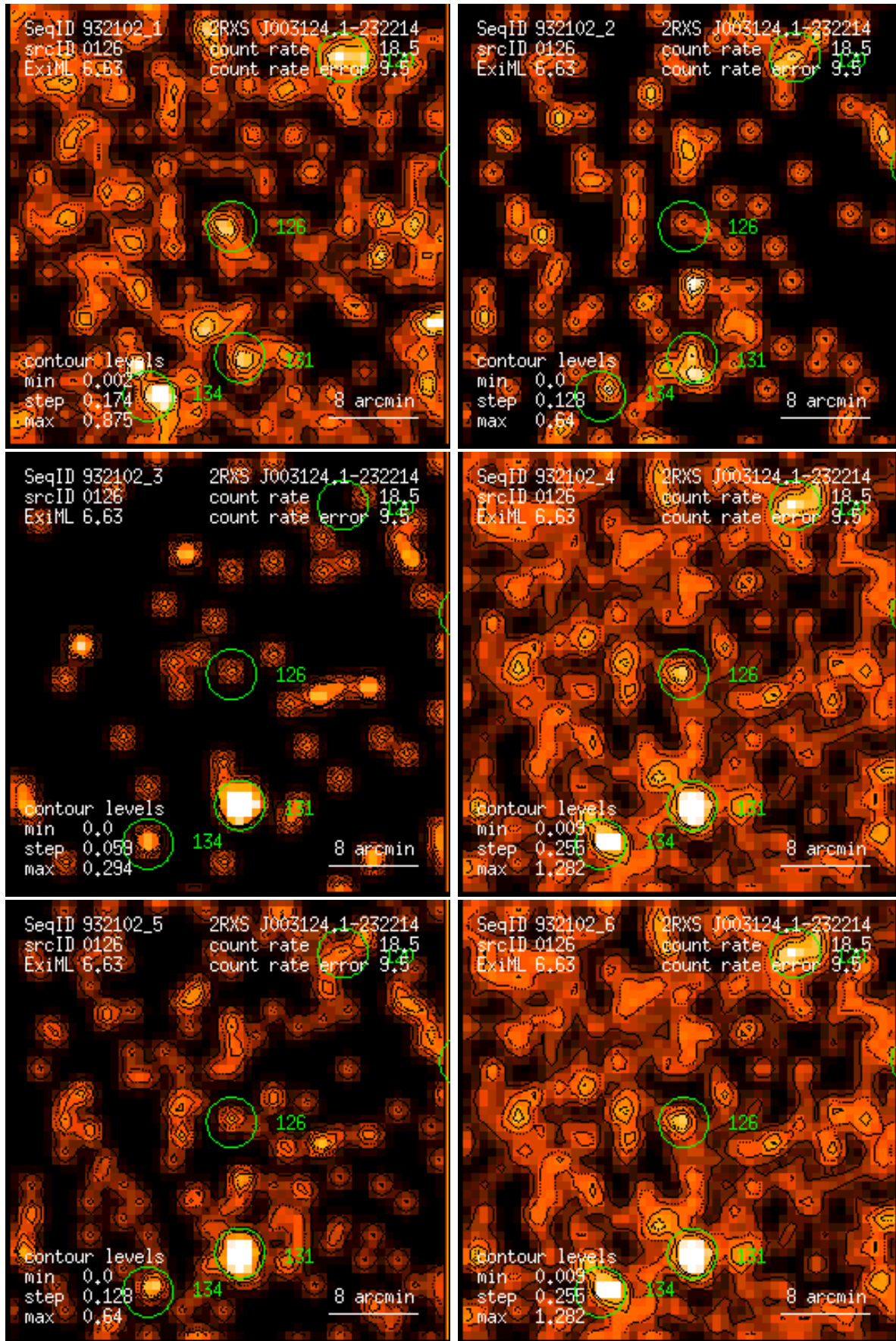
Figure 126: RASS 932102: detection 0126: band rate images, Gaussian filter: (1) PSPC channels 11 – 41, (2) 52 – 90, (3) 91 – 201, (4) 11 – 235, (5) 52 – 201, (6) 11 – 201. Broad band rates in counts/ks. Band rate contour levels in counts/ks/arcmin 2 .
