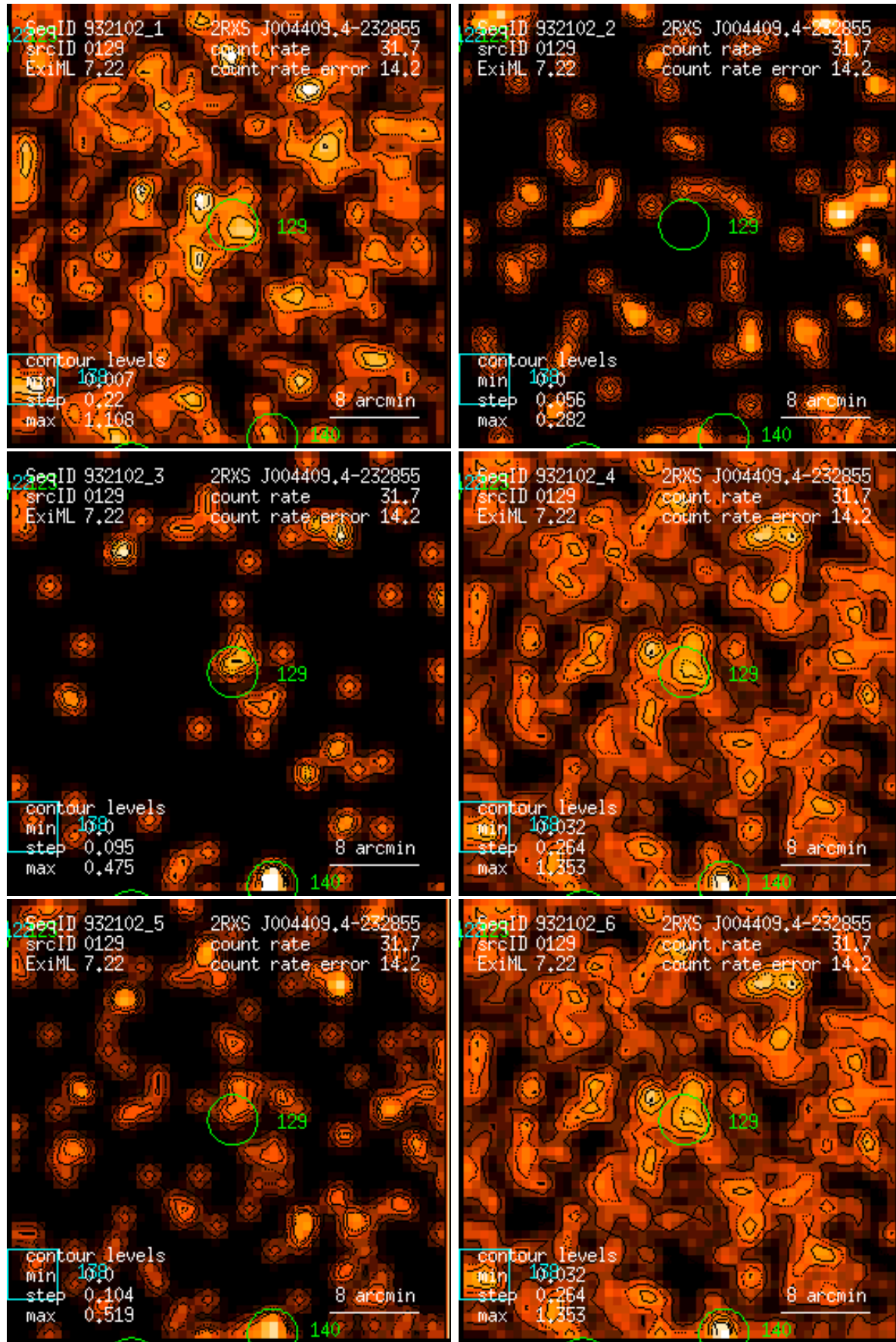
Figure 129: RASS 932102: detection 0129: band rate images, Gaussian filter: (1) PSPC channels 11 – 41, (2) 52 – 90, (3) 91 – 201, (4) 11 – 235, (5) 52 – 201, (6) 11 – 201. Broad band rates in counts/ks. Band rate contour levels in counts/ks/arcmin 2 .
