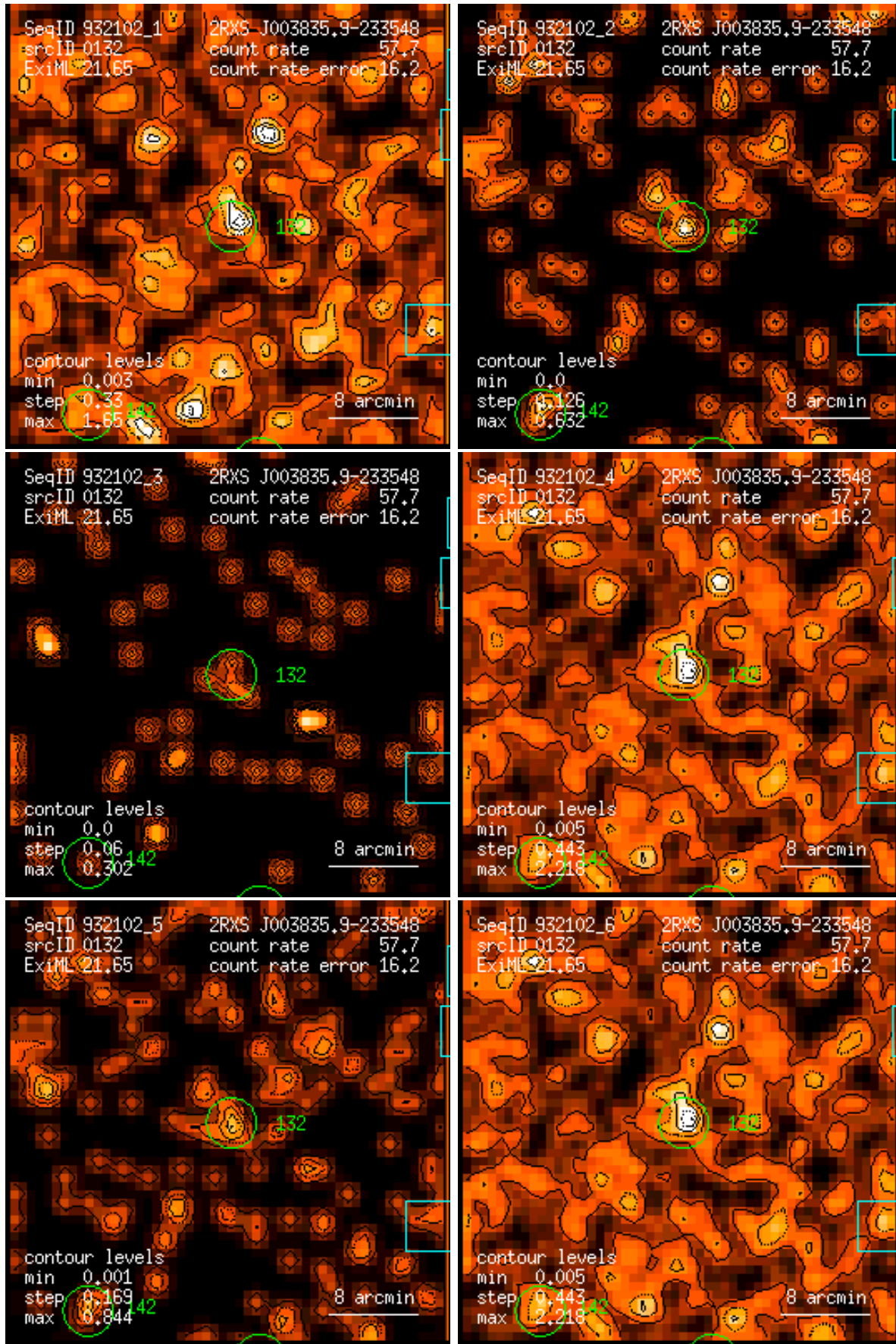
Figure 132: RASS 932102: detection 0132: band rate images, Gaussian filter: (1) PSPC channels 11 – 41, (2) 52 – 90, (3) 91 – 201, (4) 11 – 235, (5) 52 – 201, (6) 11 – 201. Broad band rates in counts/ks. Band rate contour levels in counts/ks/arcmin 2 .
