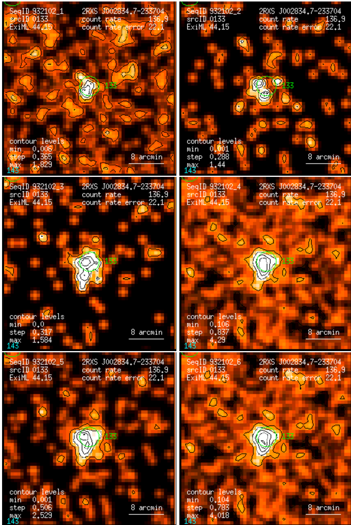
Figure 133: RASS 932102: detection 0133: band rate images, Gaussian filter: (1) PSPC channels 11 – 41, (2) 52 – 90, (3) 91 – 201, (4) 11 – 235, (5) 52 – 201, (6) 11 – 201. Broad band rates in counts/ks. Band rate contour levels in counts/ks/arcmin 2 .
