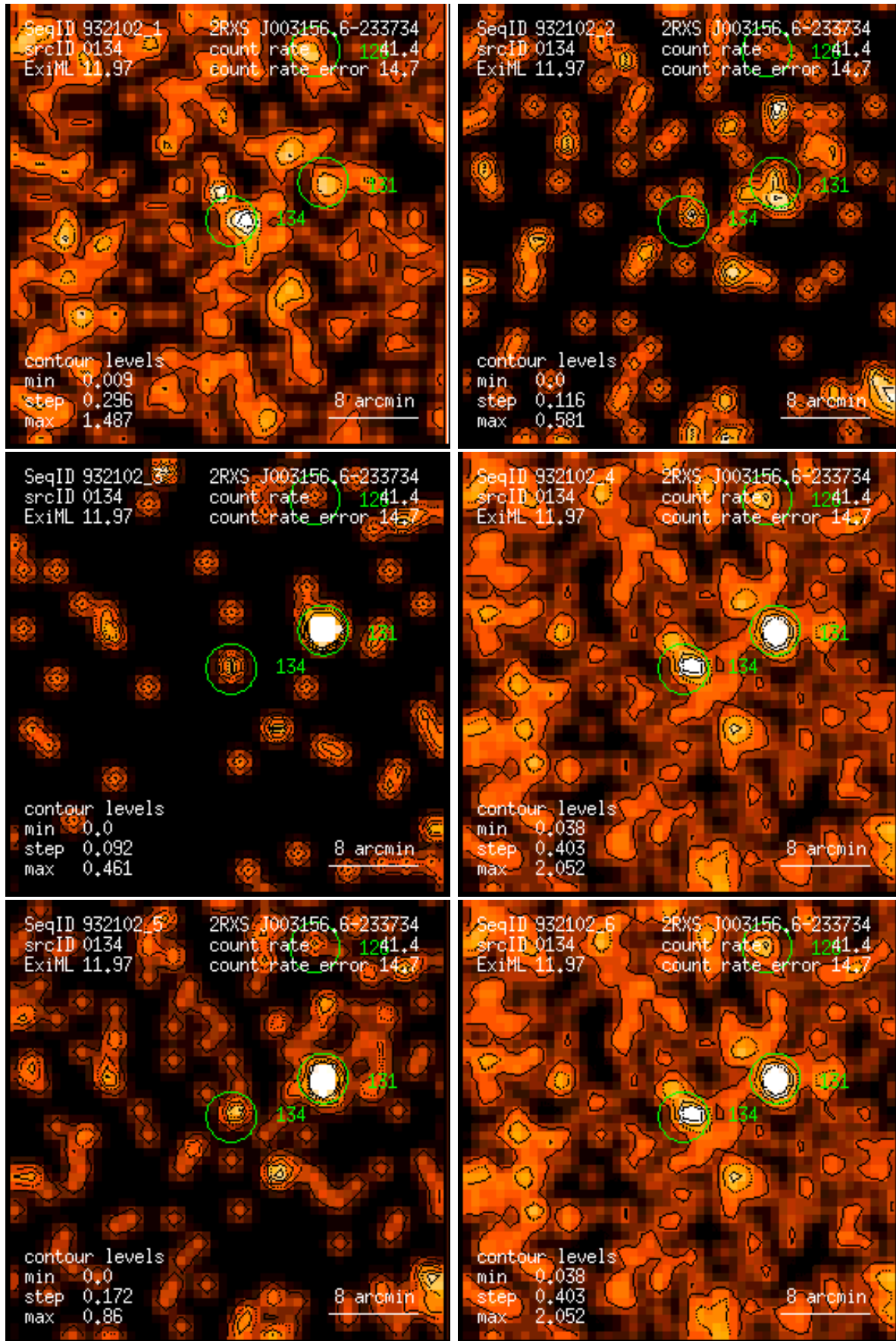
Figure 134: RASS 932102: detection 0134: band rate images, Gaussian filter: (1) PSPC channels 11 – 41, (2) 52 – 90, (3) 91 – 201, (4) 11 – 235, (5) 52 – 201, (6) 11 – 201. Broad band rates in counts/ks. Band rate contour levels in counts/ks/arcmin 2 .
