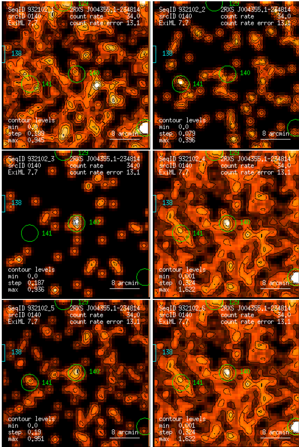
Figure 140: RASS 932102: detection 0140: band rate images, Gaussian filter: (1) PSPC channels 11 – 41, (2) 52 – 90, (3) 91 – 201, (4) 11 – 235, (5) 52 – 201, (6) 11 – 201. Broad band rates in counts/ks. Band rate contour levels in counts/ks/arcmin 2 .
