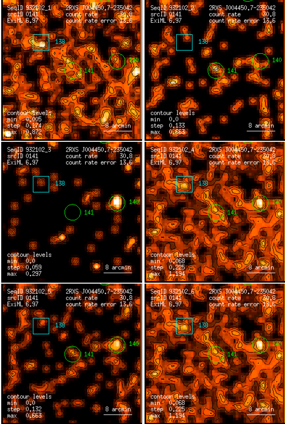
Figure 141: RASS 932102: detection 0141: band rate images, Gaussian filter: (1) PSPC channels 11 – 41, (2) 52 – 90, (3) 91 – 201, (4) 11 – 235, (5) 52 – 201, (6) 11 – 201. Broad band rates in counts/ks. Band rate contour levels in counts/ks/arcmin 2 .
