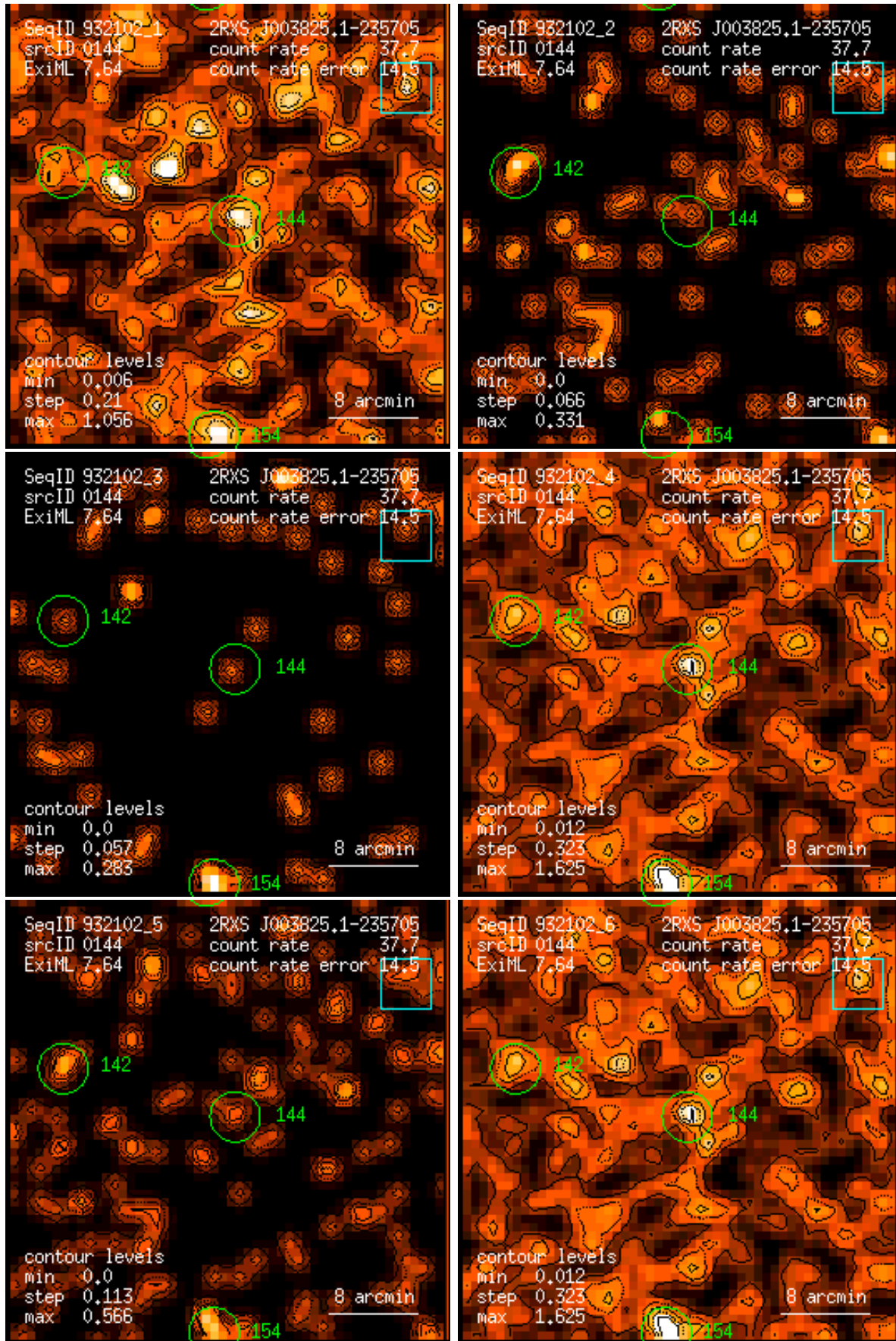
Figure 144: RASS 932102: detection 0144: band rate images, Gaussian filter: (1) PSPC channels 11 – 41, (2) 52 – 90, (3) 91 – 201, (4) 11 – 235, (5) 52 – 201, (6) 11 – 201. Broad band rates in counts/ks. Band rate contour levels in counts/ks/arcmin 2 .
