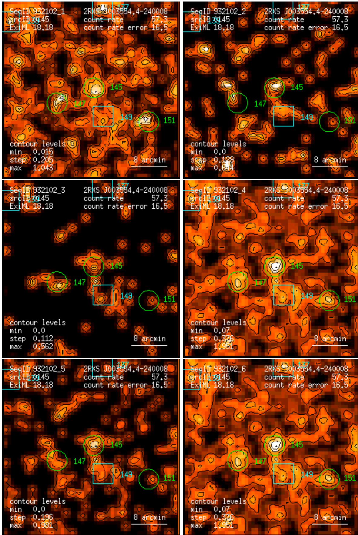
Figure 145: RASS 932102: detection 0145: band rate images, Gaussian filter: (1) PSPC channels 11 – 41, (2) 52 – 90, (3) 91 – 201, (4) 11 – 235, (5) 52 – 201, (6) 11 – 201. Broad band rates in counts/ks. Band rate contour levels in counts/ks/arcmin 2 .
