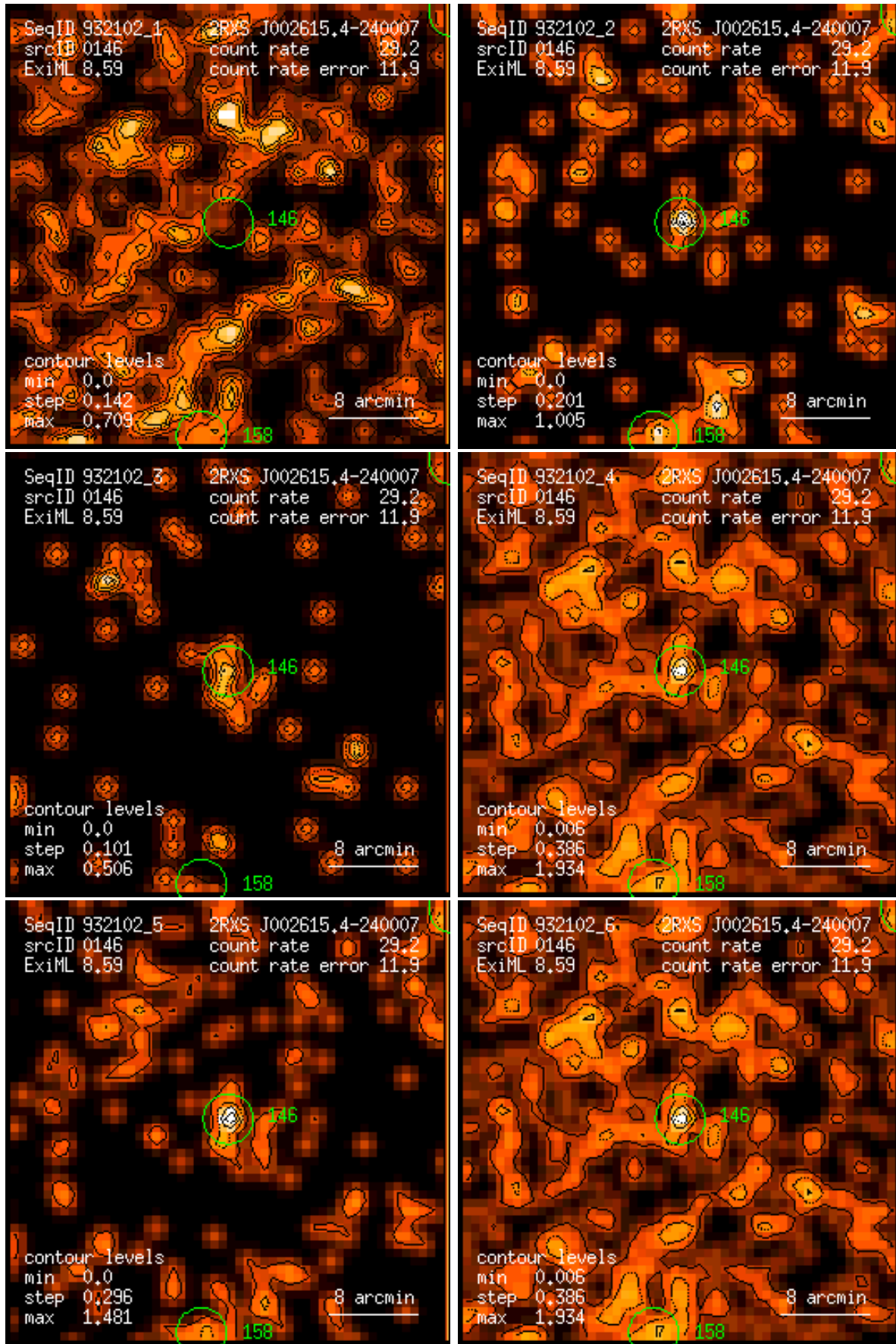
Figure 146: RASS 932102: detection 0146: band rate images, Gaussian filter: (1) PSPC channels 11 – 41, (2) 52 – 90, (3) 91 – 201, (4) 11 – 235, (5) 52 – 201, (6) 11 – 201. Broad band rates in counts/ks. Band rate contour levels in counts/ks/arcmin 2 .
