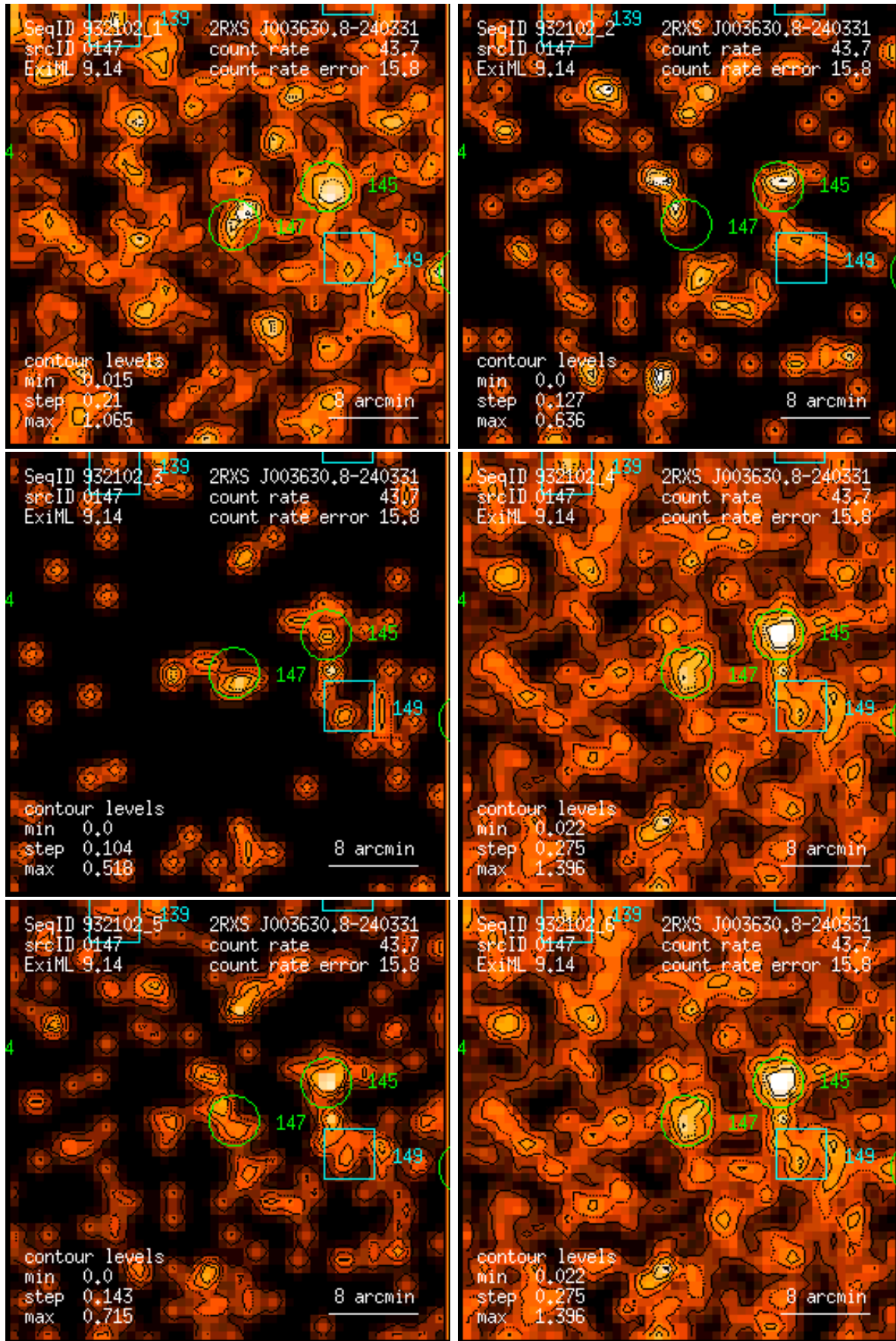
Figure 147: RASS 932102: detection 0147: band rate images, Gaussian filter: (1) PSPC channels 11 – 41, (2) 52 – 90, (3) 91 – 201, (4) 11 – 235, (5) 52 – 201, (6) 11 – 201. Broad band rates in counts/ks. Band rate contour levels in counts/ks/arcmin 2 .
