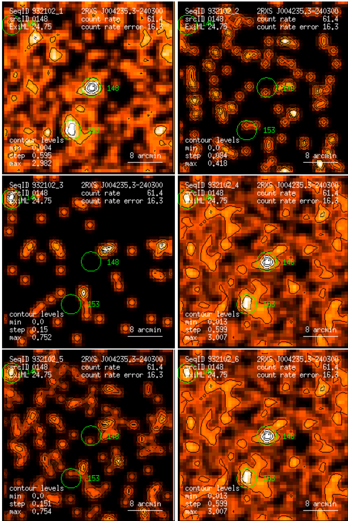
Figure 148: RASS 932102: detection 0148: band rate images, Gaussian filter: (1) PSPC channels 11 – 41, (2) 52 – 90, (3) 91 – 201, (4) 11 – 235, (5) 52 – 201, (6) 11 – 201. Broad band rates in counts/ks. Band rate contour levels in counts/ks/arcmin 2 .
