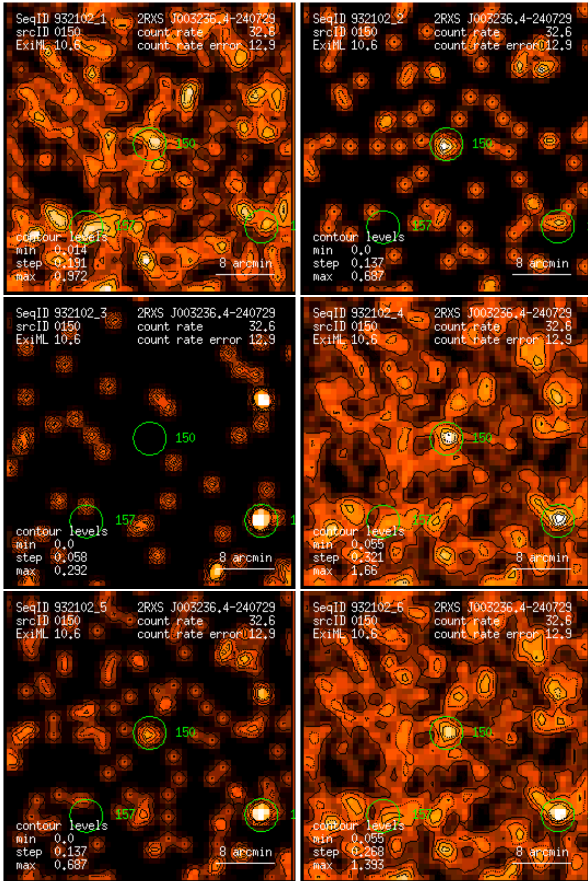
Figure 150: RASS 932102: detection 0150: band rate images, Gaussian filter: (1) PSPC channels 11 – 41, (2) 52 – 90, (3) 91 – 201, (4) 11 – 235, (5) 52 – 201, (6) 11 – 201. Broad band rates in counts/ks. Band rate contour levels in counts/ks/arcmin 2 .
