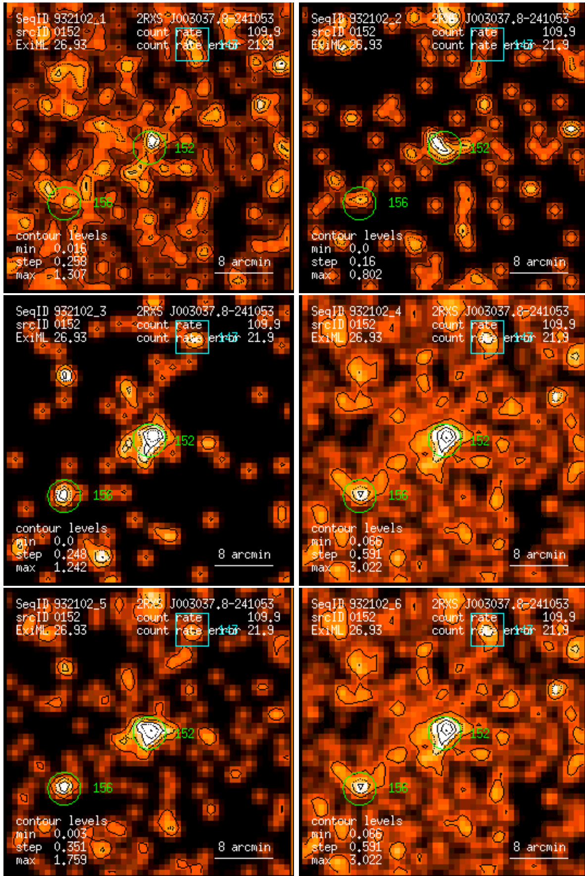
Figure 152: RASS 932102: detection 0152: band rate images, Gaussian filter: (1) PSPC channels 11 – 41, (2) 52 – 90, (3) 91 – 201, (4) 11 – 235, (5) 52 – 201, (6) 11 – 201. Broad band rates in counts/ks. Band rate contour levels in counts/ks/arcmin 2 .
