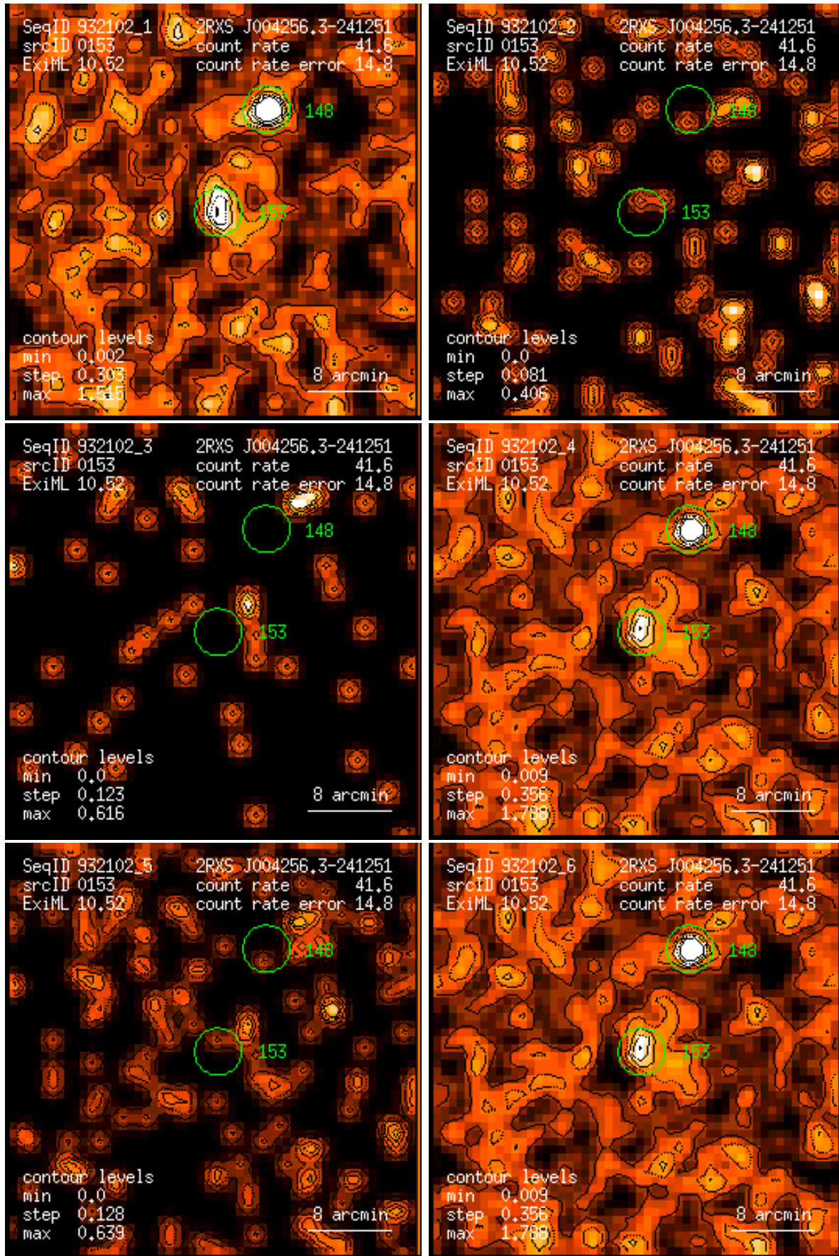
Figure 153: RASS 932102: detection 0153: band rate images, Gaussian filter: (1) PSPC channels 11 – 41, (2) 52 – 90, (3) 91 – 201, (4) 11 – 235, (5) 52 – 201, (6) 11 – 201. Broad band rates in counts/ks. Band rate contour levels in counts/ks/arcmin 2 .
