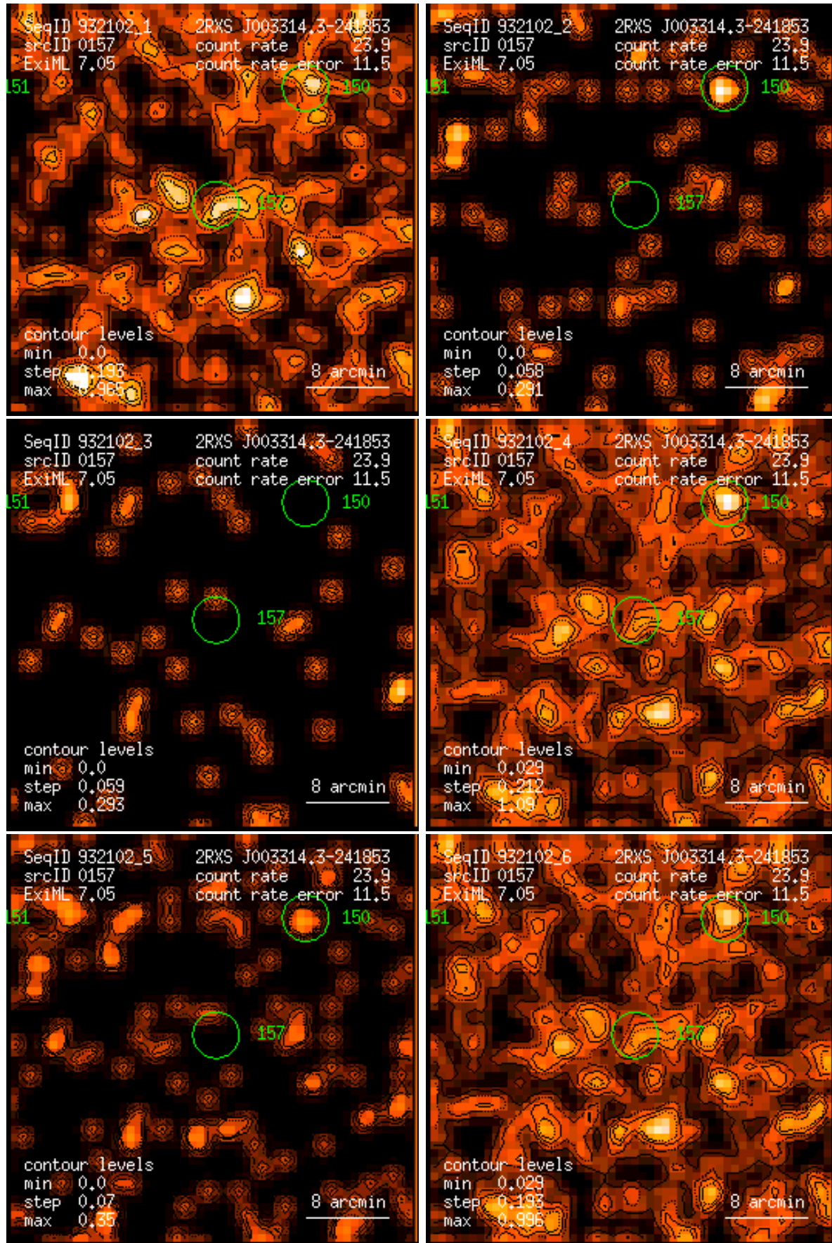
Figure 157: RASS 932102: detection 0157: band rate images, Gaussian filter: (1) PSPC channels 11 – 41, (2) 52 – 90, (3) 91 – 201, (4) 11 – 235, (5) 52 – 201, (6) 11 – 201. Broad band rates in counts/ks. Band rate contour levels in counts/ks/arcmin 2 .
