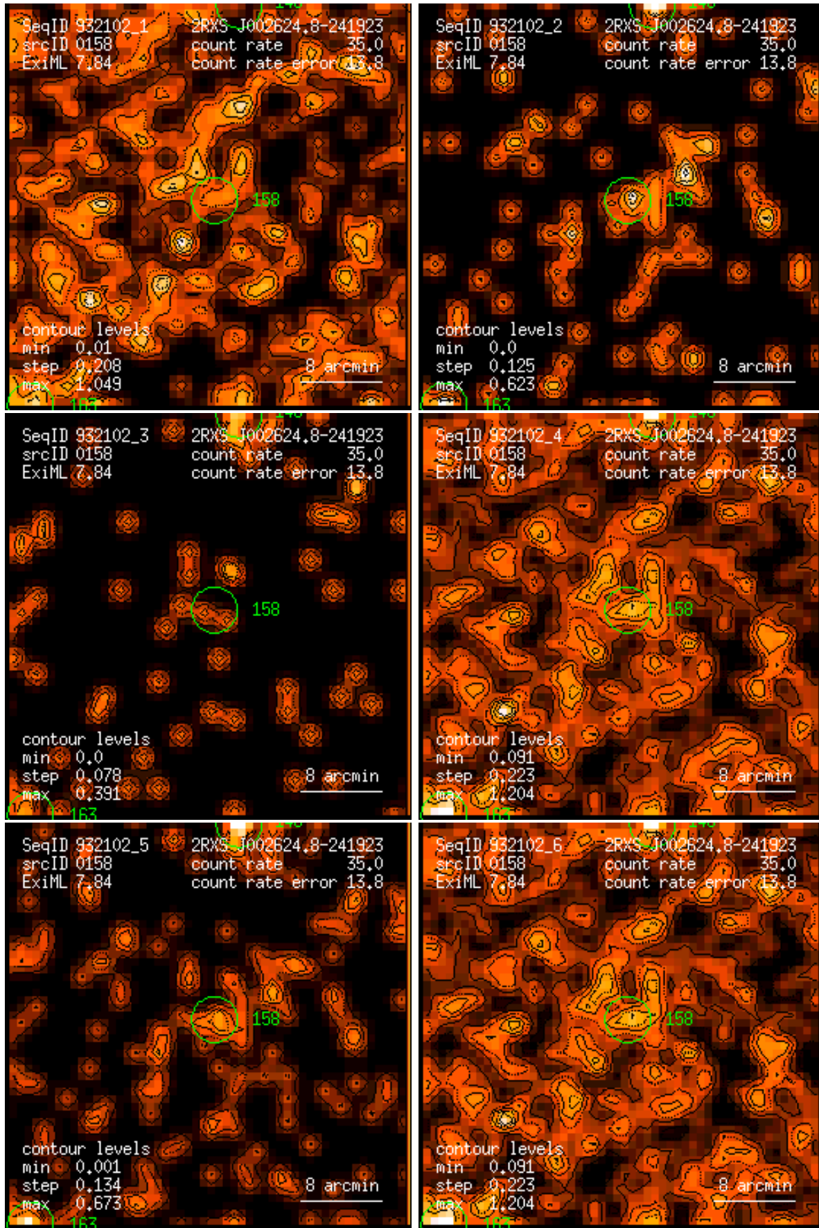
Figure 158: RASS 932102: detection 0158: band rate images, Gaussian filter: (1) PSPC channels 11 – 41, (2) 52 – 90, (3) 91 – 201, (4) 11 – 235, (5) 52 – 201, (6) 11 – 201. Broad band rates in counts/ks. Band rate contour levels in counts/ks/arcmin 2 .
