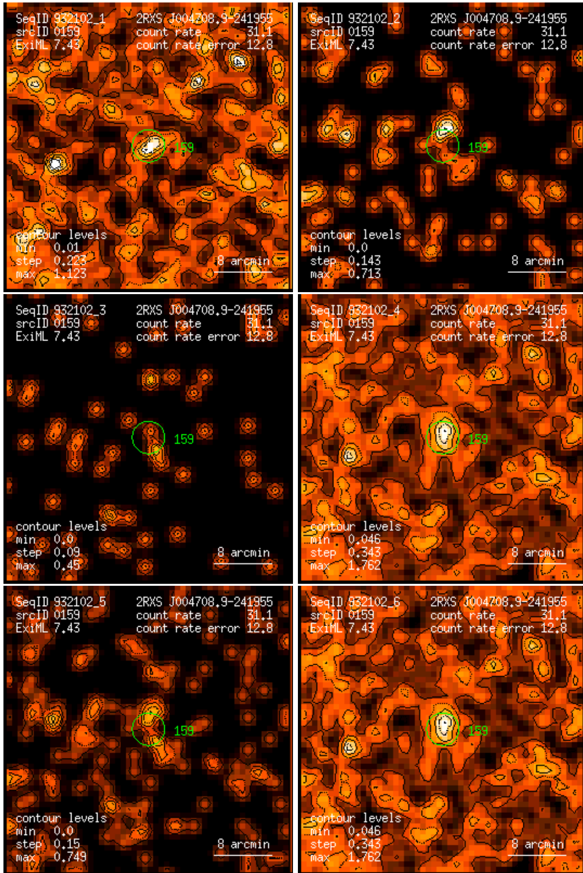
Figure 159: RASS 932102: detection 0159: band rate images, Gaussian filter: (1) PSPC channels 11 – 41, (2) 52 – 90, (3) 91 – 201, (4) 11 – 235, (5) 52 – 201, (6) 11 – 201. Broad band rates in counts/ks. Band rate contour levels in counts/ks/arcmin 2 .
