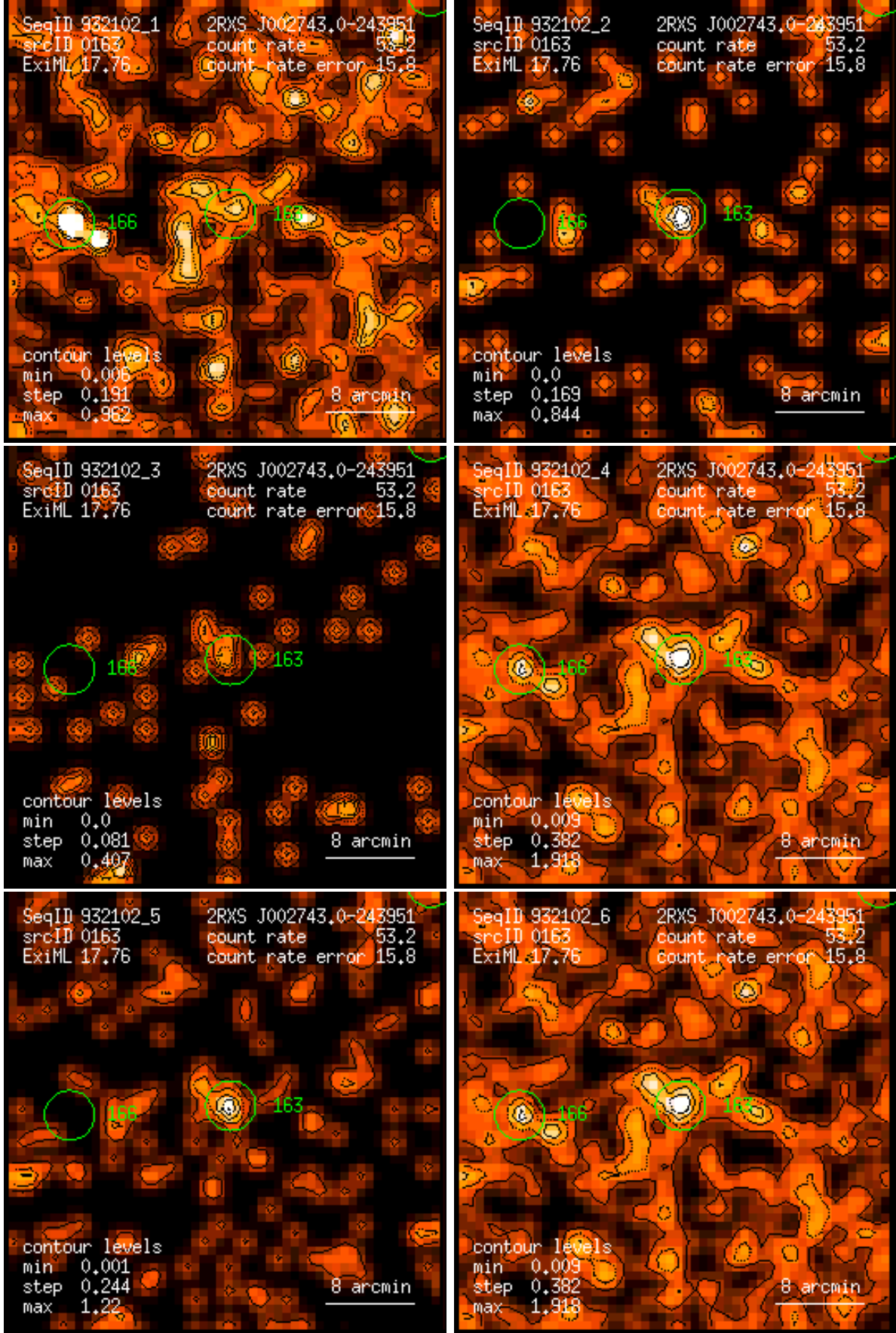
Figure 163: RASS 932102: detection 0163: band rate images, Gaussian filter: (1) PSPC channels 11 – 41, (2) 52 – 90, (3) 91 – 201, (4) 11 – 235, (5) 52 – 201, (6) 11 – 201. Broad band rates in counts/ks. Band rate contour levels in counts/ks/arcmin 2 .
