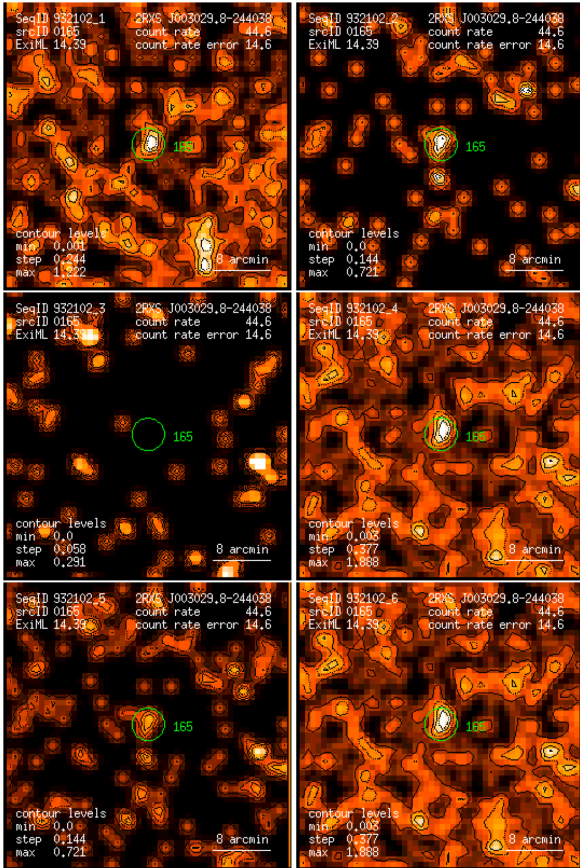
Figure 165: RASS 932102: detection 0165: band rate images, Gaussian filter: (1) PSPC channels 11 – 41, (2) 52 – 90, (3) 91 – 201, (4) 11 – 235, (5) 52 – 201, (6) 11 – 201. Broad band rates in counts/ks. Band rate contour levels in counts/ks/arcmin 2 .
