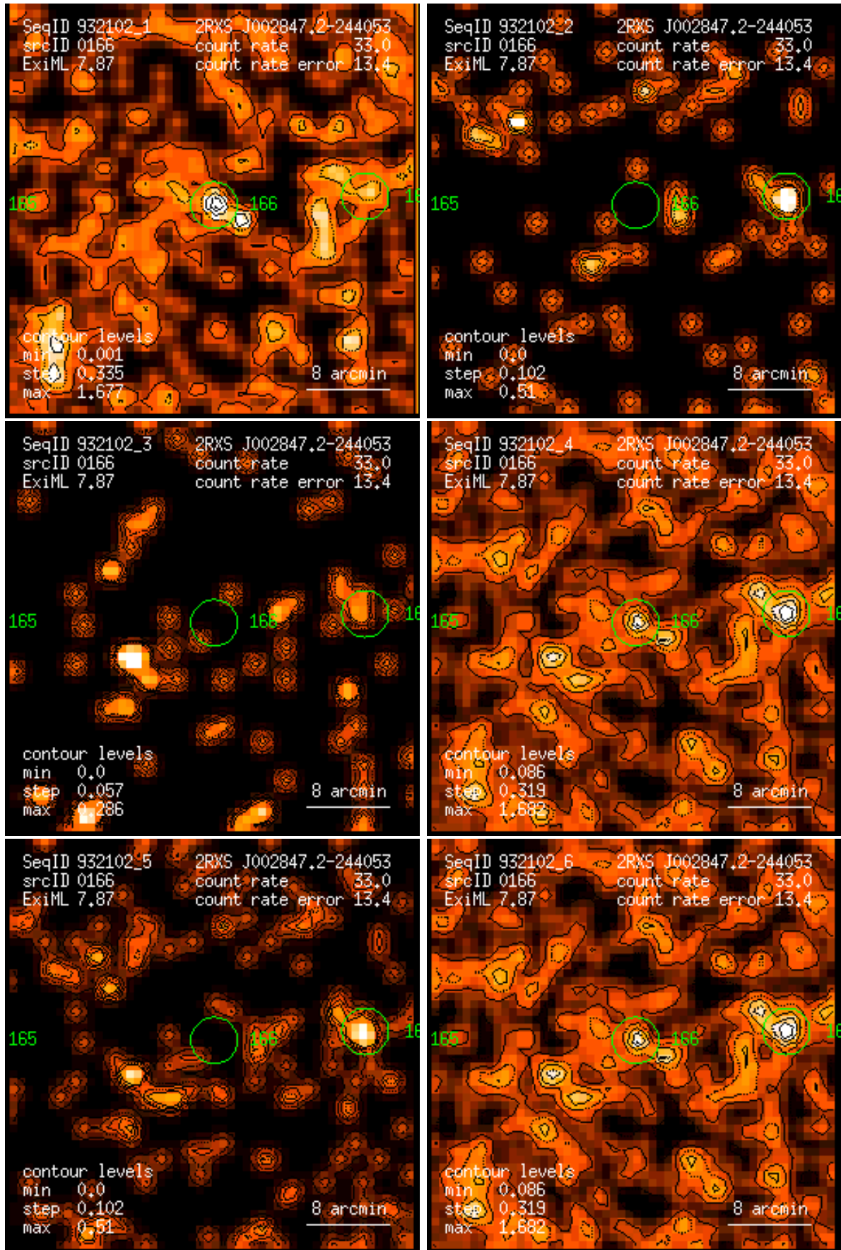
Figure 166: RASS 932102: detection 0166: band rate images, Gaussian filter: (1) PSPC channels 11 – 41, (2) 52 – 90, (3) 91 – 201, (4) 11 – 235, (5) 52 – 201, (6) 11 – 201. Broad band rates in counts/ks. Band rate contour levels in counts/ks/arcmin 2 .
