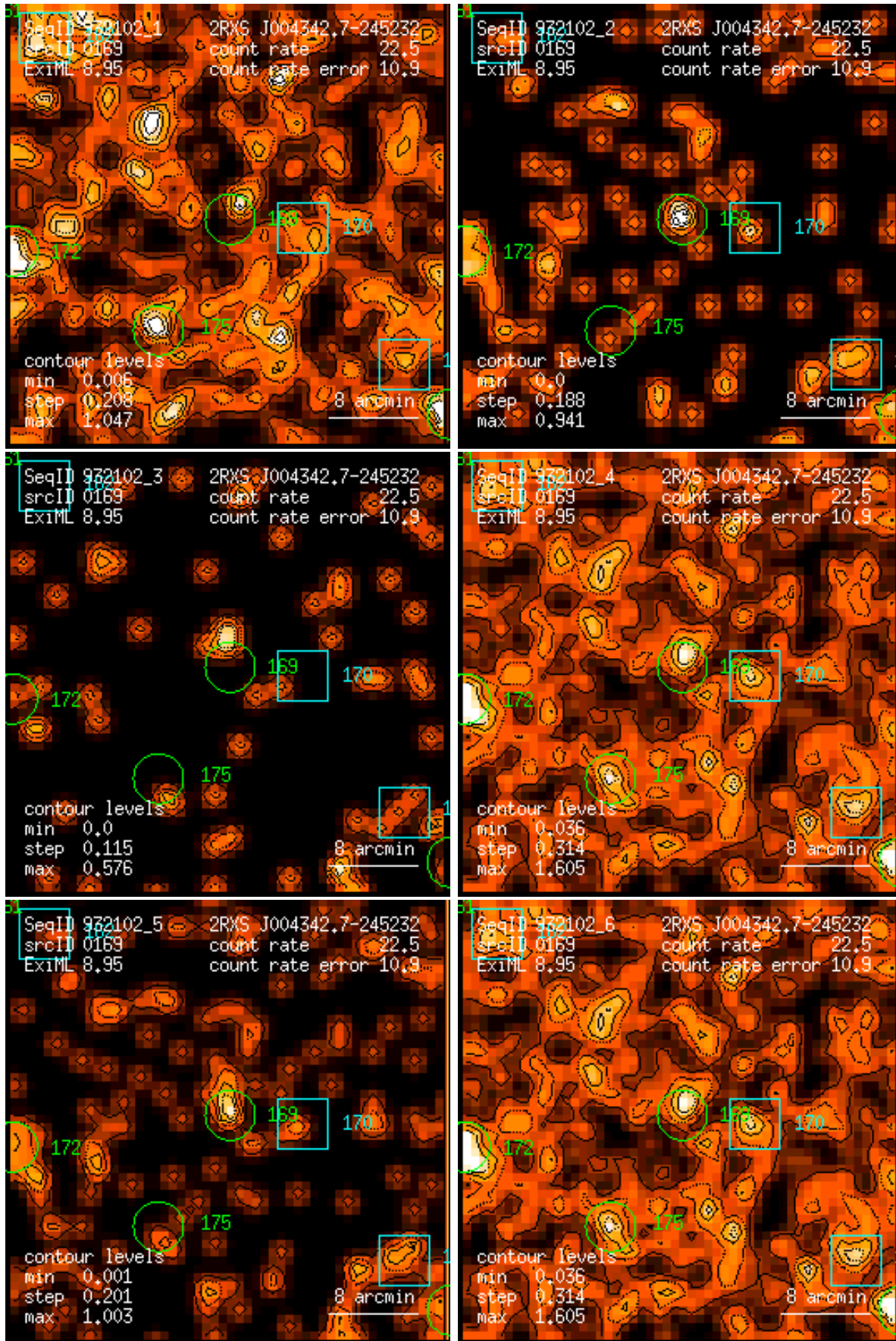
Figure 169: RASS 932102: detection 0169: band rate images, Gaussian filter: (1) PSPC channels 11 – 41, (2) 52 – 90, (3) 91 – 201, (4) 11 – 235, (5) 52 – 201, (6) 11 – 201. Broad band rates in counts/ks. Band rate contour levels in counts/ks/arcmin 2 .
