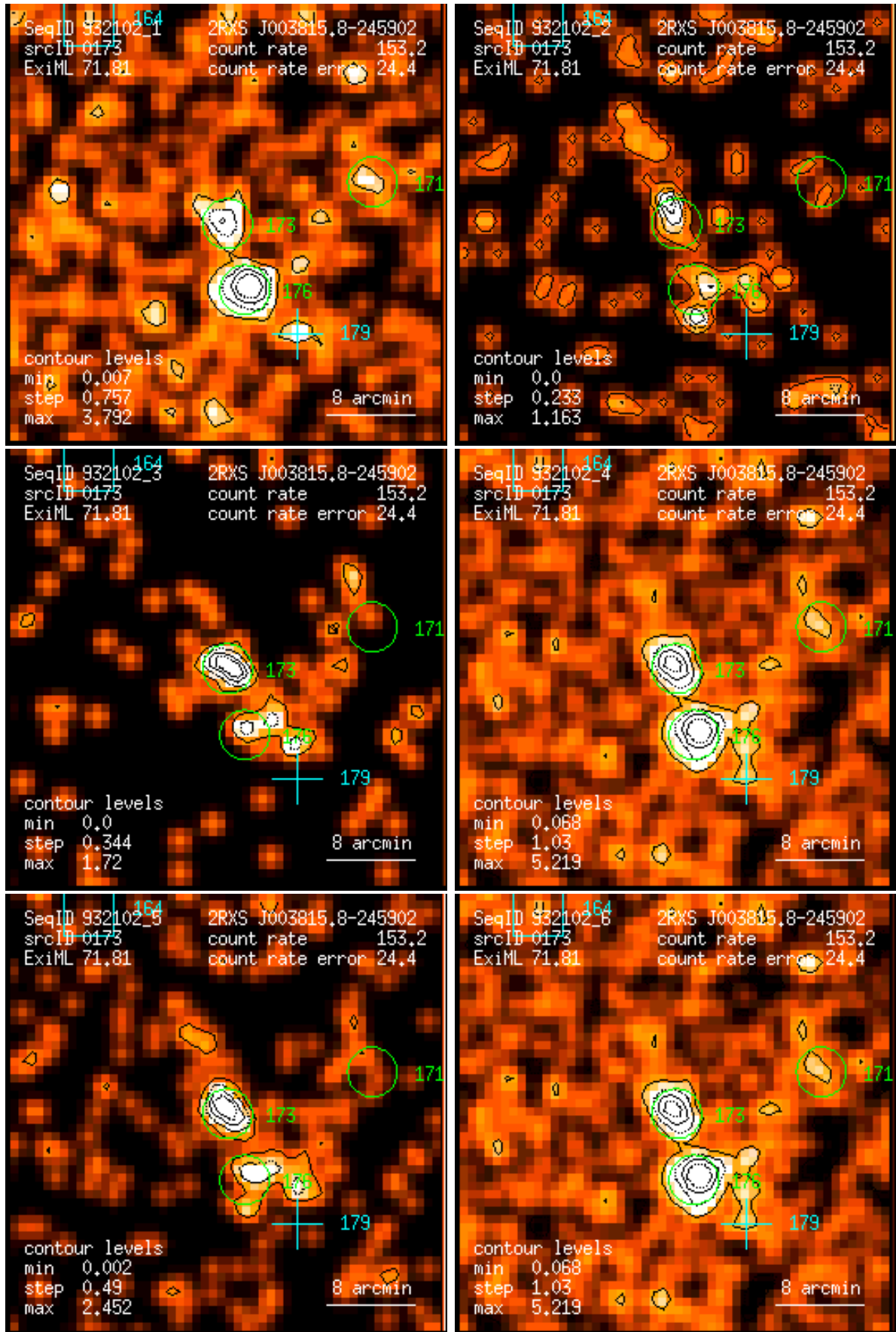
Figure 173: RASS 932102: detection 0173: band rate images, Gaussian filter: (1) PSPC channels 11 – 41, (2) 52 – 90, (3) 91 – 201, (4) 11 – 235, (5) 52 – 201, (6) 11 – 201. Broad band rates in counts/ks. Band rate contour levels in counts/ks/arcmin 2 .
