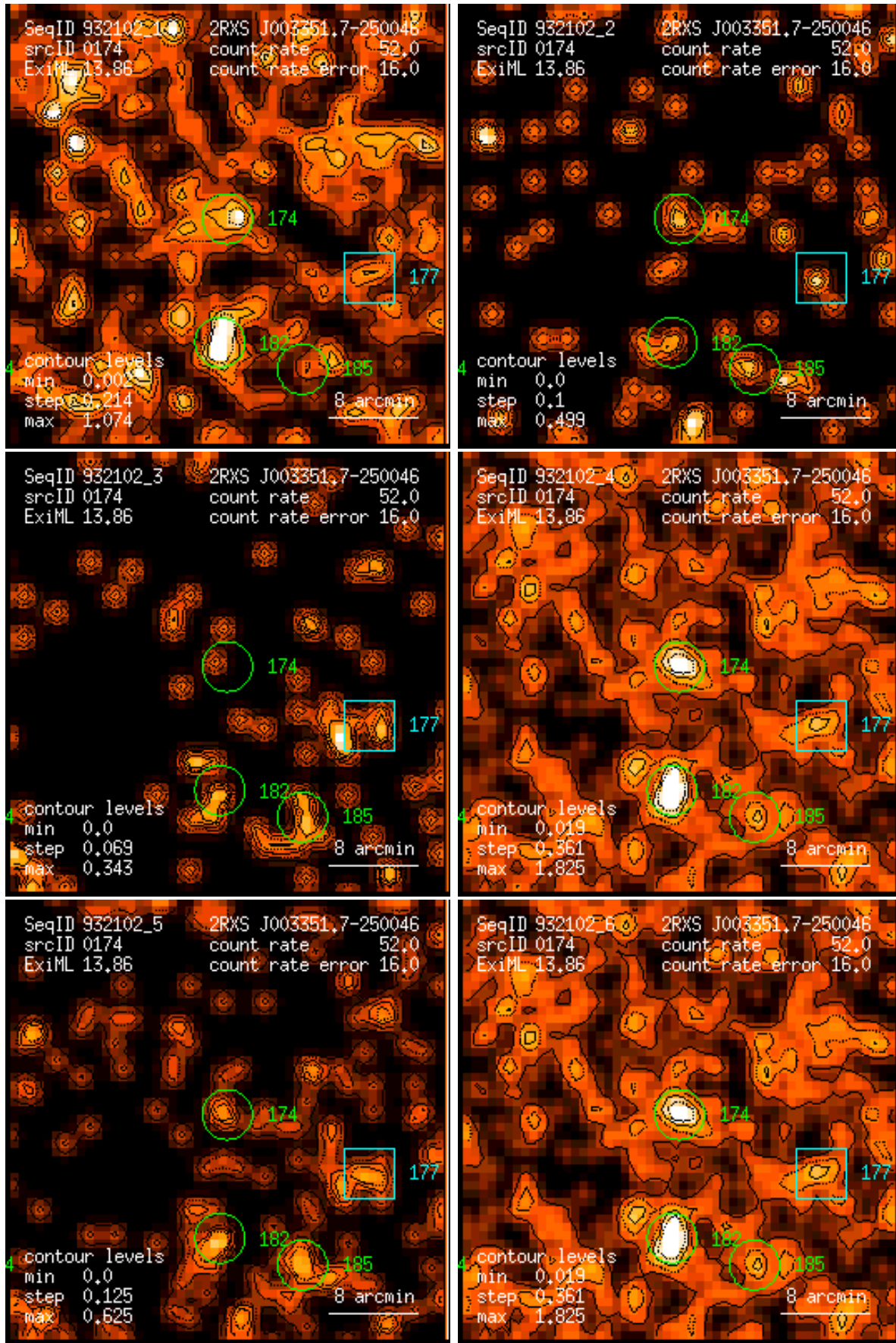
Figure 174: RASS 932102: detection 0174: band rate images, Gaussian filter: (1) PSPC channels 11 – 41, (2) 52 – 90, (3) 91 – 201, (4) 11 – 235, (5) 52 – 201, (6) 11 – 201. Broad band rates in counts/ks. Band rate contour levels in counts/ks/arcmin 2 .
