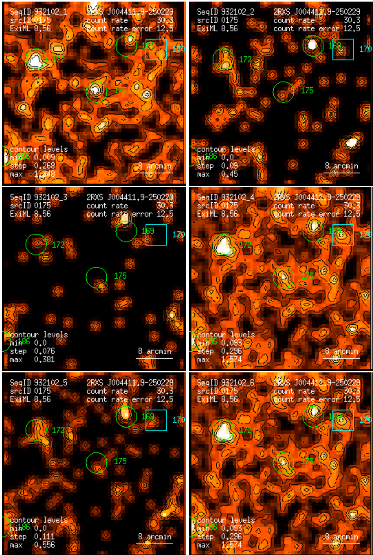
Figure 175: RASS 932102: detection 0175: band rate images, Gaussian filter: (1) PSPC channels 11 – 41, (2) 52 – 90, (3) 91 – 201, (4) 11 – 235, (5) 52 – 201, (6) 11 – 201. Broad band rates in counts/ks. Band rate contour levels in counts/ks/arcmin 2 .
