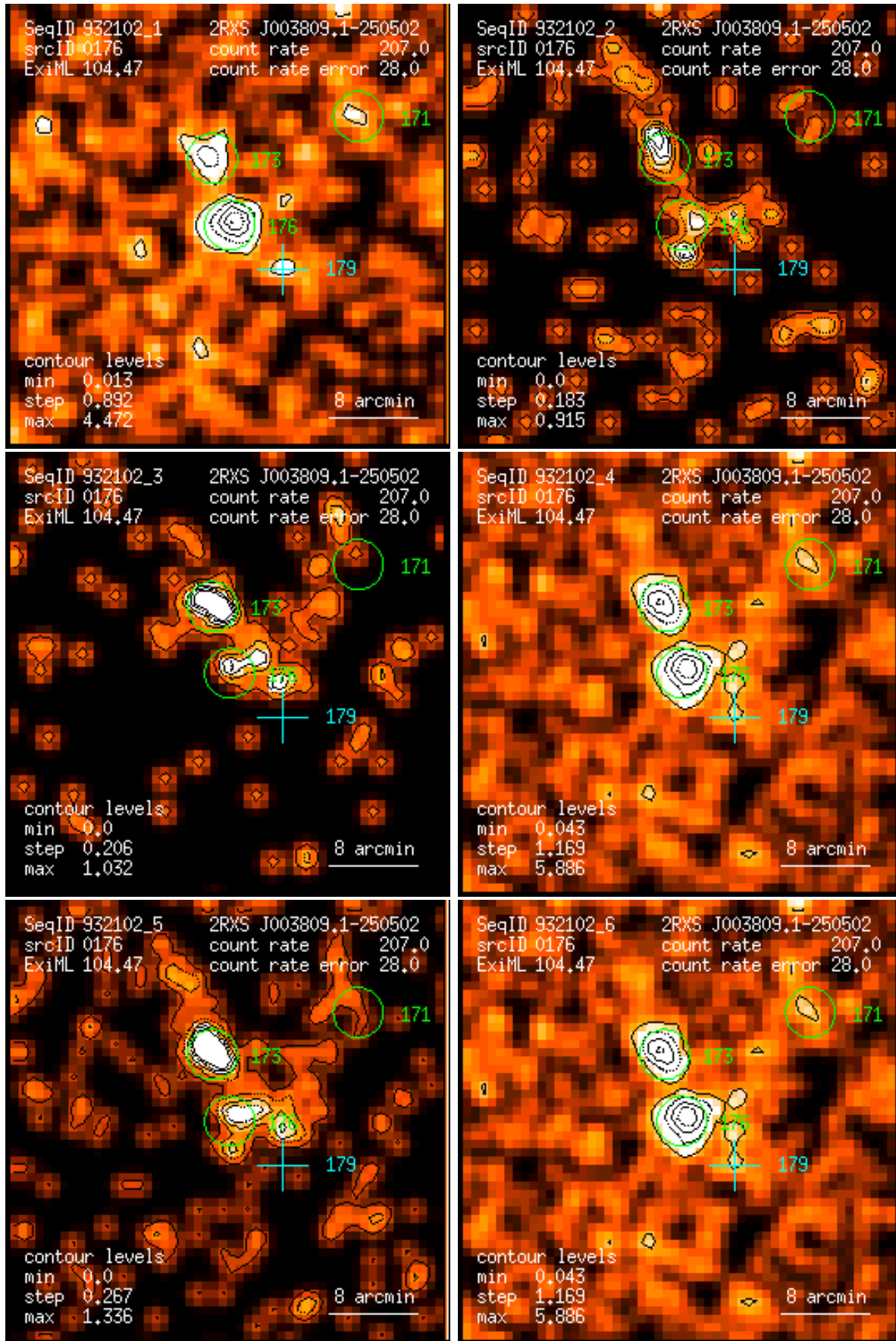
Figure 176: RASS 932102: detection 0176: band rate images, Gaussian filter: (1) PSPC channels 11 – 41, (2) 52 – 90, (3) 91 – 201, (4) 11 – 235, (5) 52 – 201, (6) 11 – 201. Broad band rates in counts/ks. Band rate contour levels in counts/ks/arcmin 2 .
