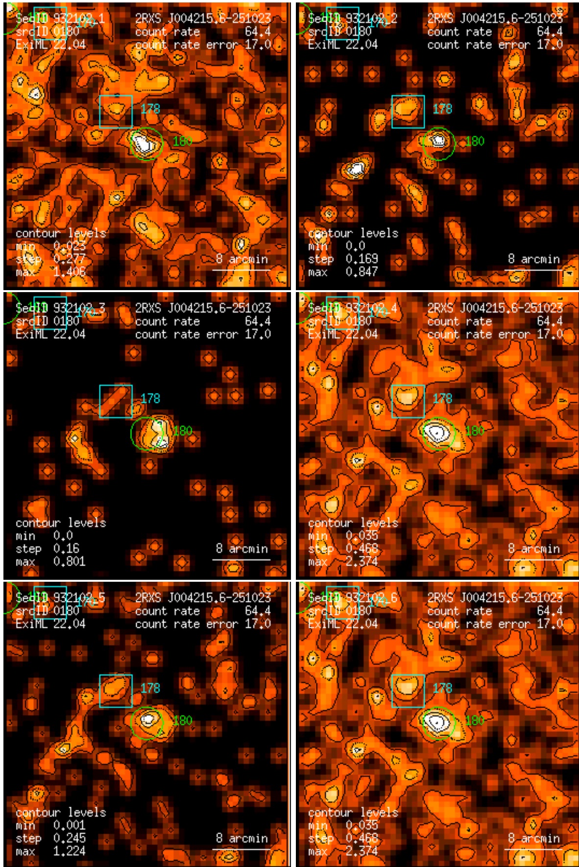
Figure 180: RASS 932102: detection 0180: band rate images, Gaussian filter: (1) PSPC channels 11 – 41, (2) 52 – 90, (3) 91 – 201, (4) 11 – 235, (5) 52 – 201, (6) 11 – 201. Broad band rates in counts/ks. Band rate contour levels in counts/ks/arcmin 2 .
