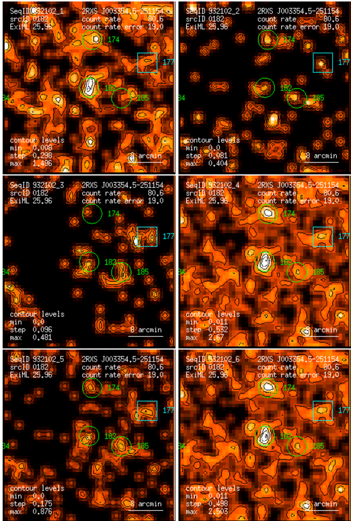
Figure 182: RASS 932102: detection 0182: band rate images, Gaussian filter: (1) PSPC channels 11 – 41, (2) 52 – 90, (3) 91 – 201, (4) 11 – 235, (5) 52 – 201, (6) 11 – 201. Broad band rates in counts/ks. Band rate contour levels in counts/ks/arcmin 2 .
