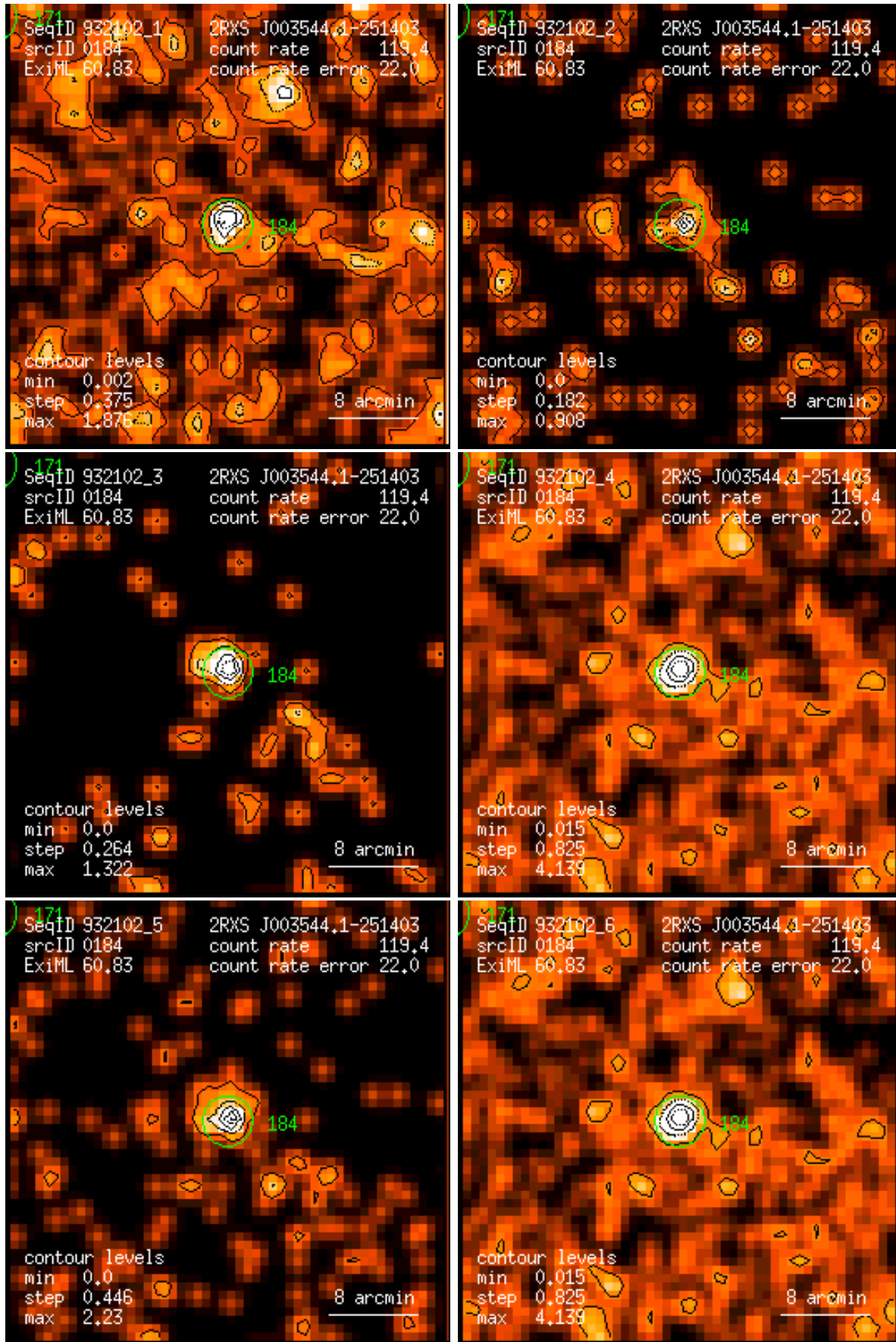
Figure 184: RASS 932102: detection 0184: band rate images, Gaussian filter: (1) PSPC channels 11 – 41, (2) 52 – 90, (3) 91 – 201, (4) 11 – 235, (5) 52 – 201, (6) 11 – 201. Broad band rates in counts/ks. Band rate contour levels in counts/ks/arcmin 2 .
