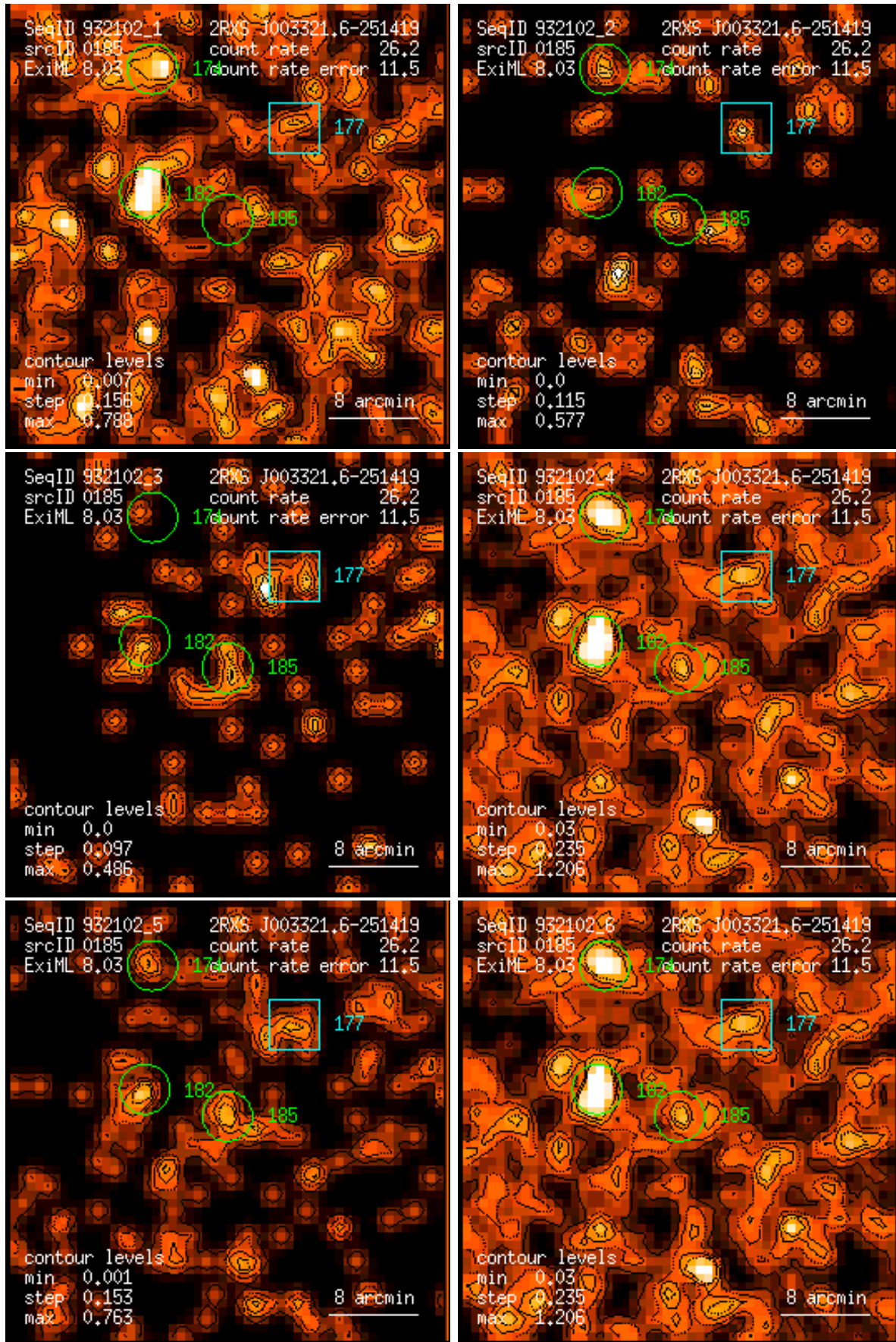
Figure 185: RASS 932102: detection 0185: band rate images, Gaussian filter: (1) PSPC channels 11 – 41, (2) 52 – 90, (3) 91 – 201, (4) 11 – 235, (5) 52 – 201, (6) 11 – 201. Broad band rates in counts/ks. Band rate contour levels in counts/ks/arcmin 2 .
