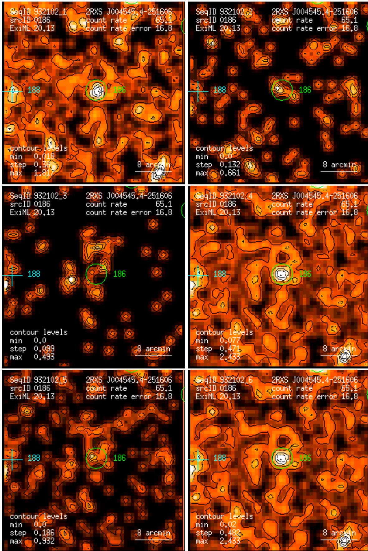
Figure 186: RASS 932102: detection 0186: band rate images, Gaussian filter: (1) PSPC channels 11 – 41, (2) 52 – 90, (3) 91 – 201, (4) 11 – 235, (5) 52 – 201, (6) 11 – 201. Broad band rates in counts/ks. Band rate contour levels in counts/ks/arcmin 2 .
