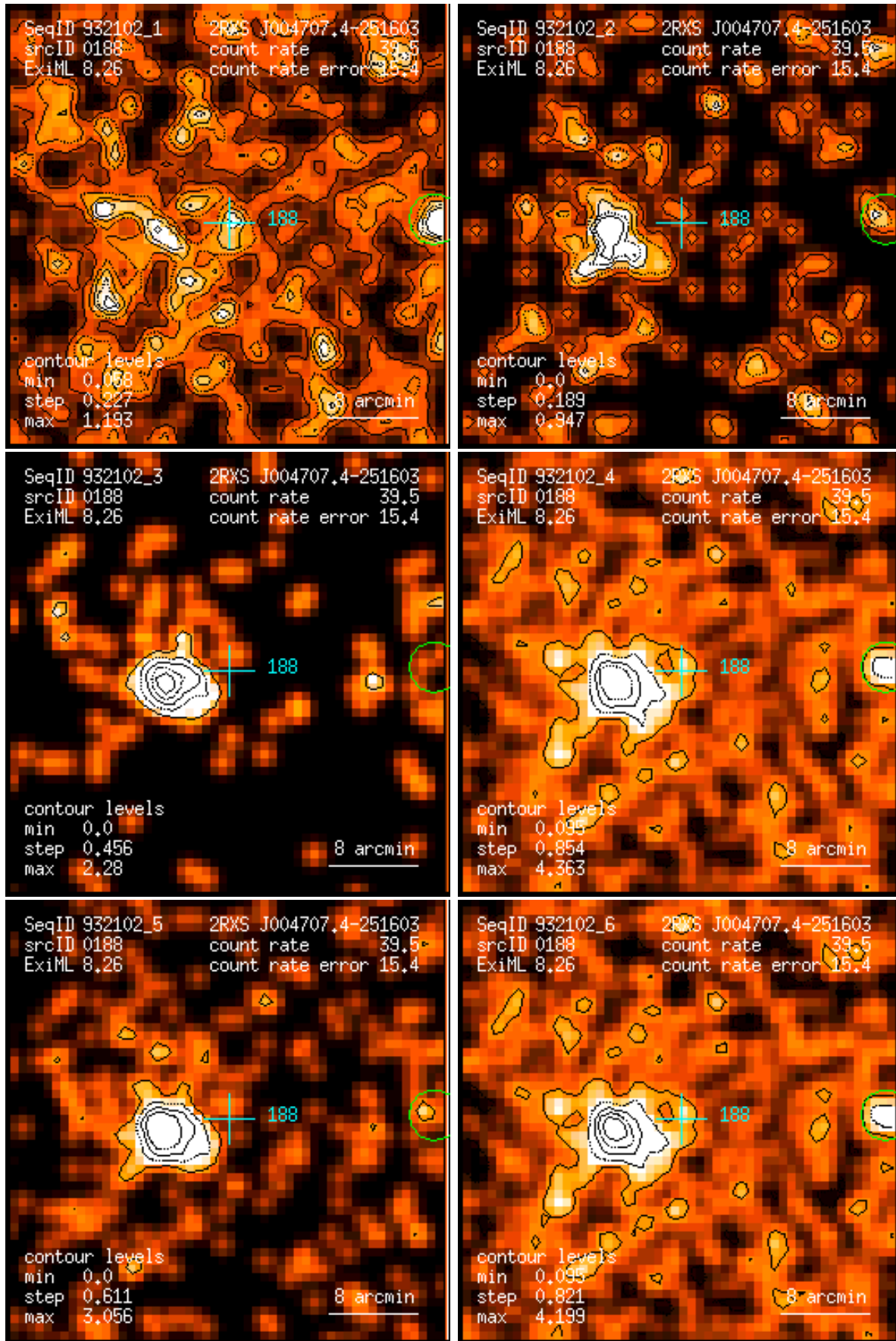
Figure 188: RASS 932102: detection 0188: band rate images, Gaussian filter: (1) PSPC channels 11 – 41, (2) 52 – 90, (3) 91 – 201, (4) 11 – 235, (5) 52 – 201, (6) 11 – 201. Broad band rates in counts/ks. Band rate contour levels in counts/ks/arcmin 2 .
