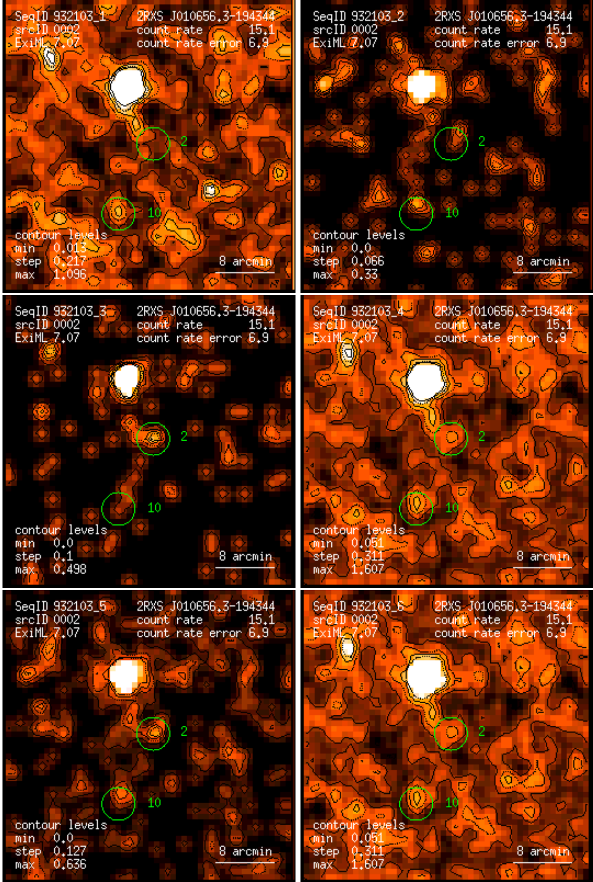
Figure 2: RASS 932103: detection 0002: band rate images, Gaussian filter: (1) PSPC channels 11 – 41, (2) 52 – 90, (3) 91 – 201, (4) 11 – 235, (5) 52 – 201, (6) 11 – 201. Broad band rates in counts/ks. Band rate contour levels in counts/ks/arcmin 2 .
