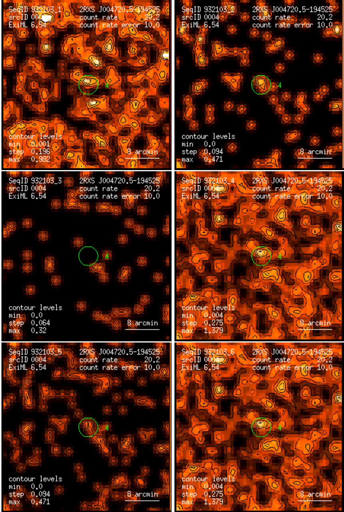
Figure 4: RASS 932103: detection 0004: band rate images, Gaussian filter: (1) PSPC channels 11 – 41, (2) 52 – 90, (3) 91 – 201, (4) 11 – 235, (5) 52 – 201, (6) 11 – 201. Broad band rates in counts/ks. Band rate contour levels in counts/ks/arcmin 2 .
