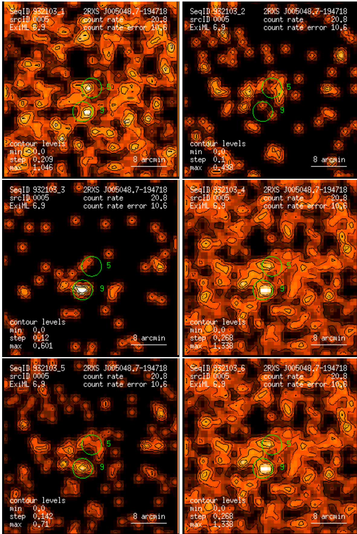
Figure 5: RASS 932103: detection 0005: band rate images, Gaussian filter: (1) PSPC channels 11 – 41, (2) 52 – 90, (3) 91 – 201, (4) 11 – 235, (5) 52 – 201, (6) 11 – 201. Broad band rates in counts/ks. Band rate contour levels in counts/ks/arcmin 2 .
