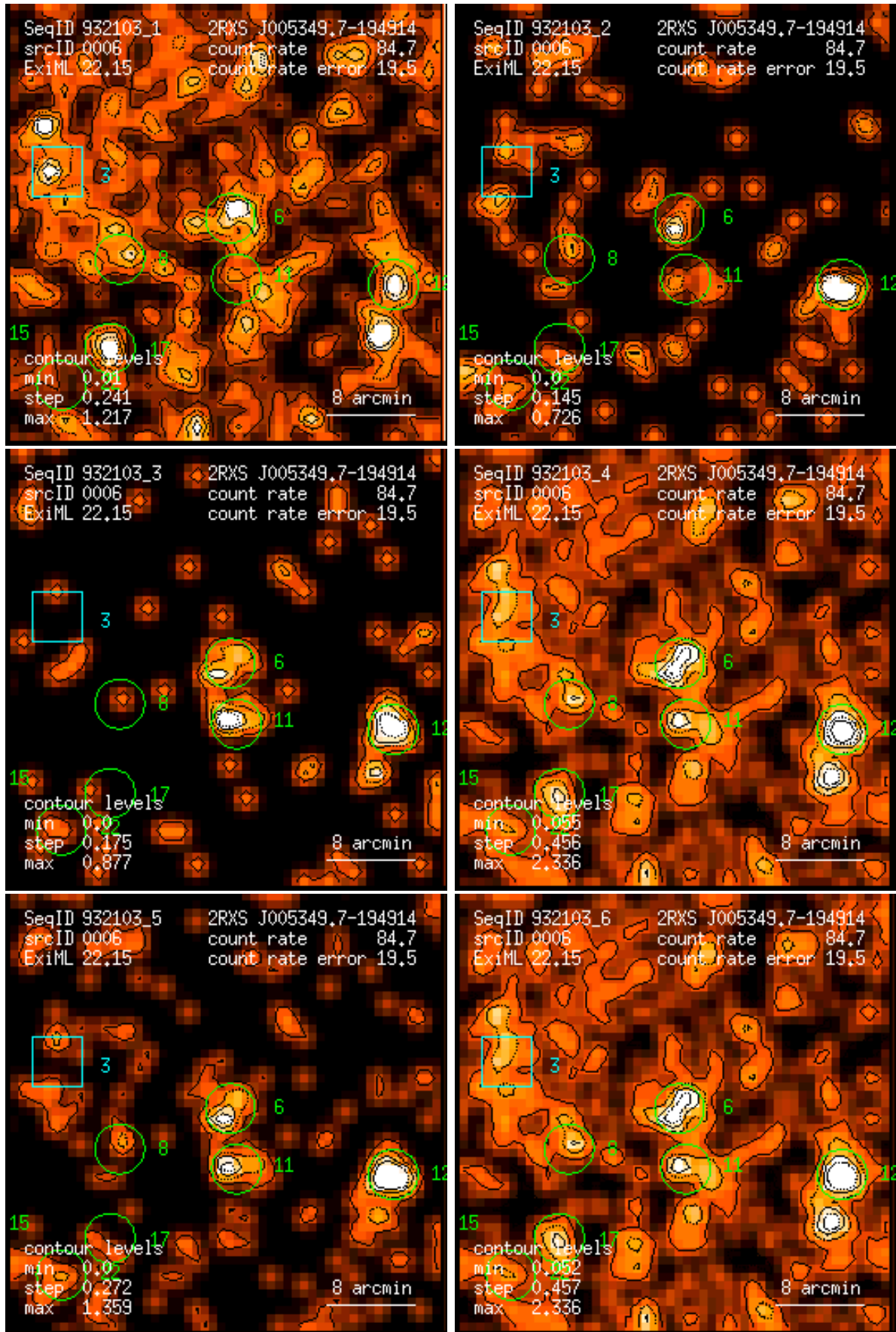
Figure 6: RASS 932103: detection 0006: band rate images, Gaussian filter: (1) PSPC channels 11 – 41, (2) 52 – 90, (3) 91 – 201, (4) 11 – 235, (5) 52 – 201, (6) 11 – 201. Broad band rates in counts/ks. Band rate contour levels in counts/ks/arcmin 2 .
