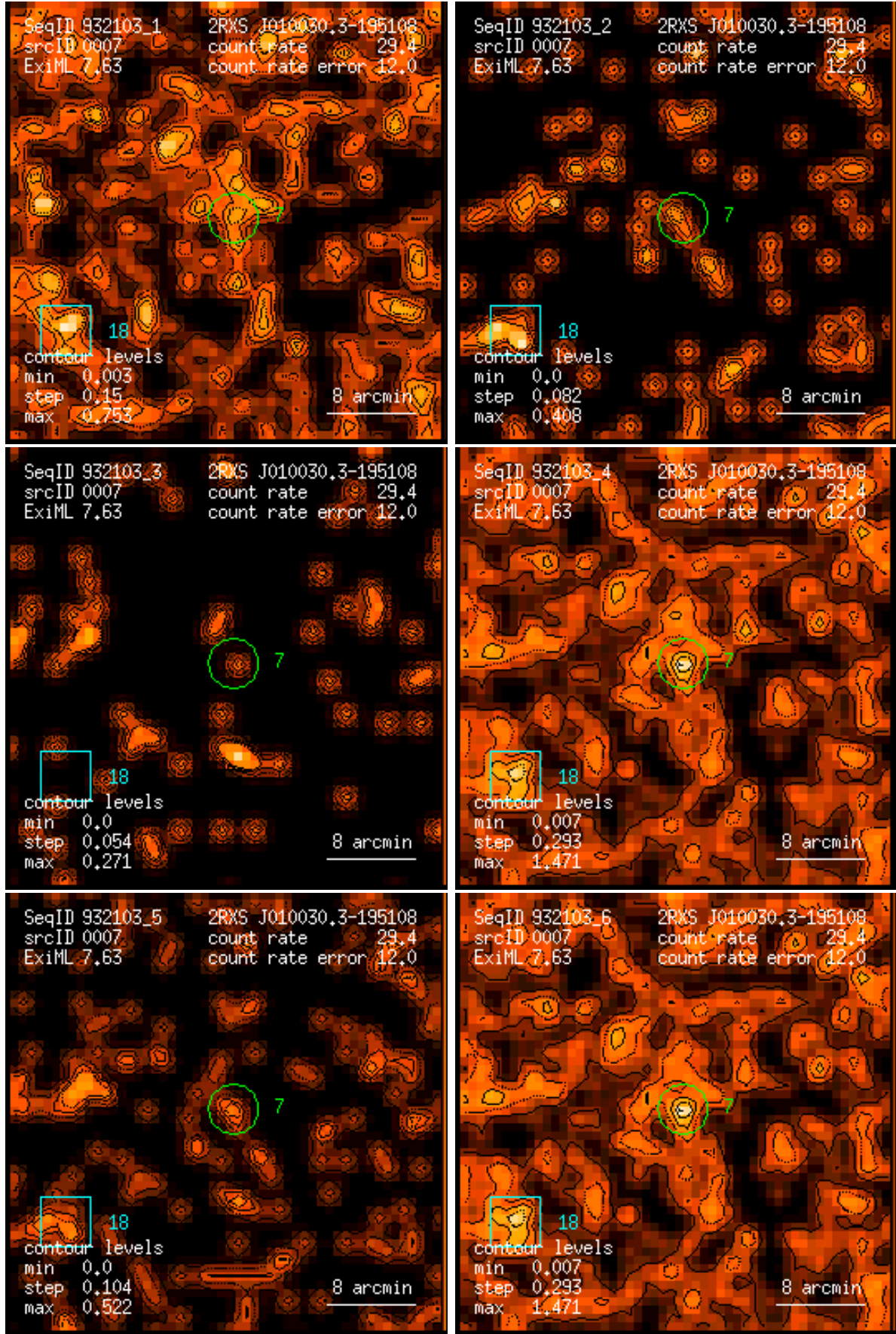
Figure 7: RASS 932103: detection 0007: band rate images, Gaussian filter: (1) PSPC channels 11 – 41, (2) 52 – 90, (3) 91 – 201, (4) 11 – 235, (5) 52 – 201, (6) 11 – 201. Broad band rates in counts/ks. Band rate contour levels in counts/ks/arcmin 2 .
