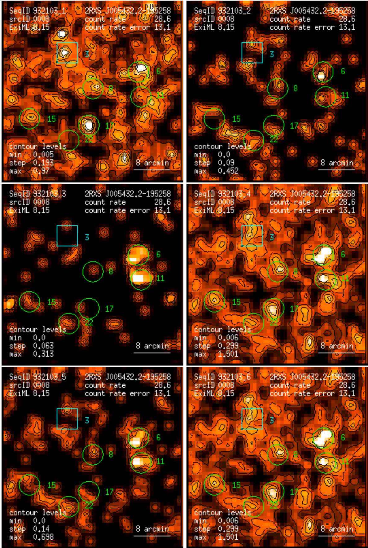
Figure 8: RASS 932103: detection 0008: band rate images, Gaussian filter: (1) PSPC channels 11 – 41, (2) 52 – 90, (3) 91 – 201, (4) 11 – 235, (5) 52 – 201, (6) 11 – 201. Broad band rates in counts/ks. Band rate contour levels in counts/ks/arcmin 2 .
