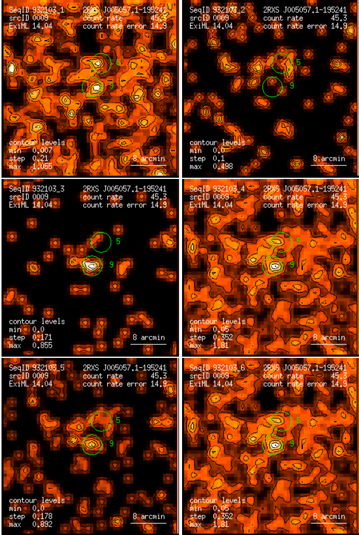
Figure 9: RASS 932103: detection 0009: band rate images, Gaussian filter: (1) PSPC channels 11 – 41, (2) 52 – 90, (3) 91 – 201, (4) 11 – 235, (5) 52 – 201, (6) 11 – 201. Broad band rates in counts/ks. Band rate contour levels in counts/ks/arcmin 2 .
