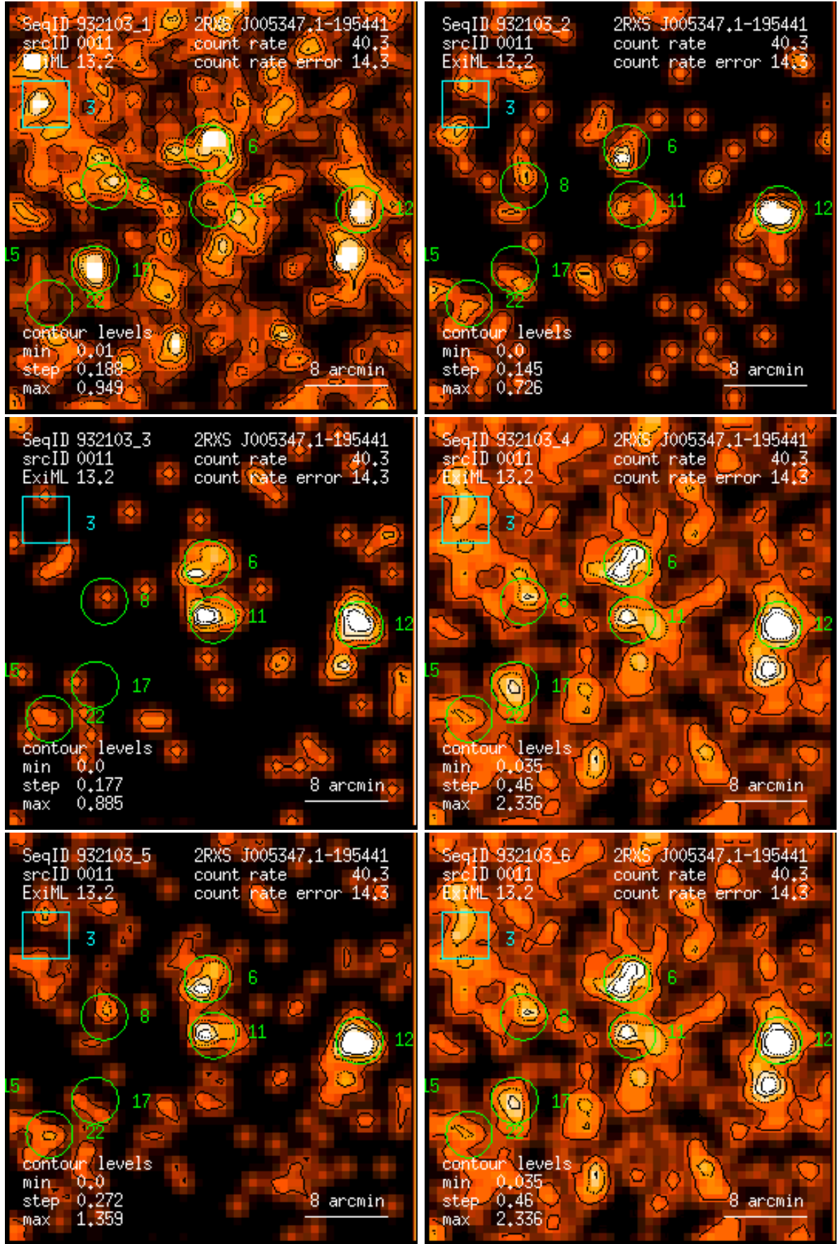
Figure 11: RASS 932103: detection 0011: band rate images, Gaussian filter: (1) PSPC channels 11 – 41, (2) 52 – 90, (3) 91 – 201, (4) 11 – 235, (5) 52 – 201, (6) 11 – 201. Broad band rates in counts/ks. Band rate contour levels in counts/ks/arcmin 2 .
