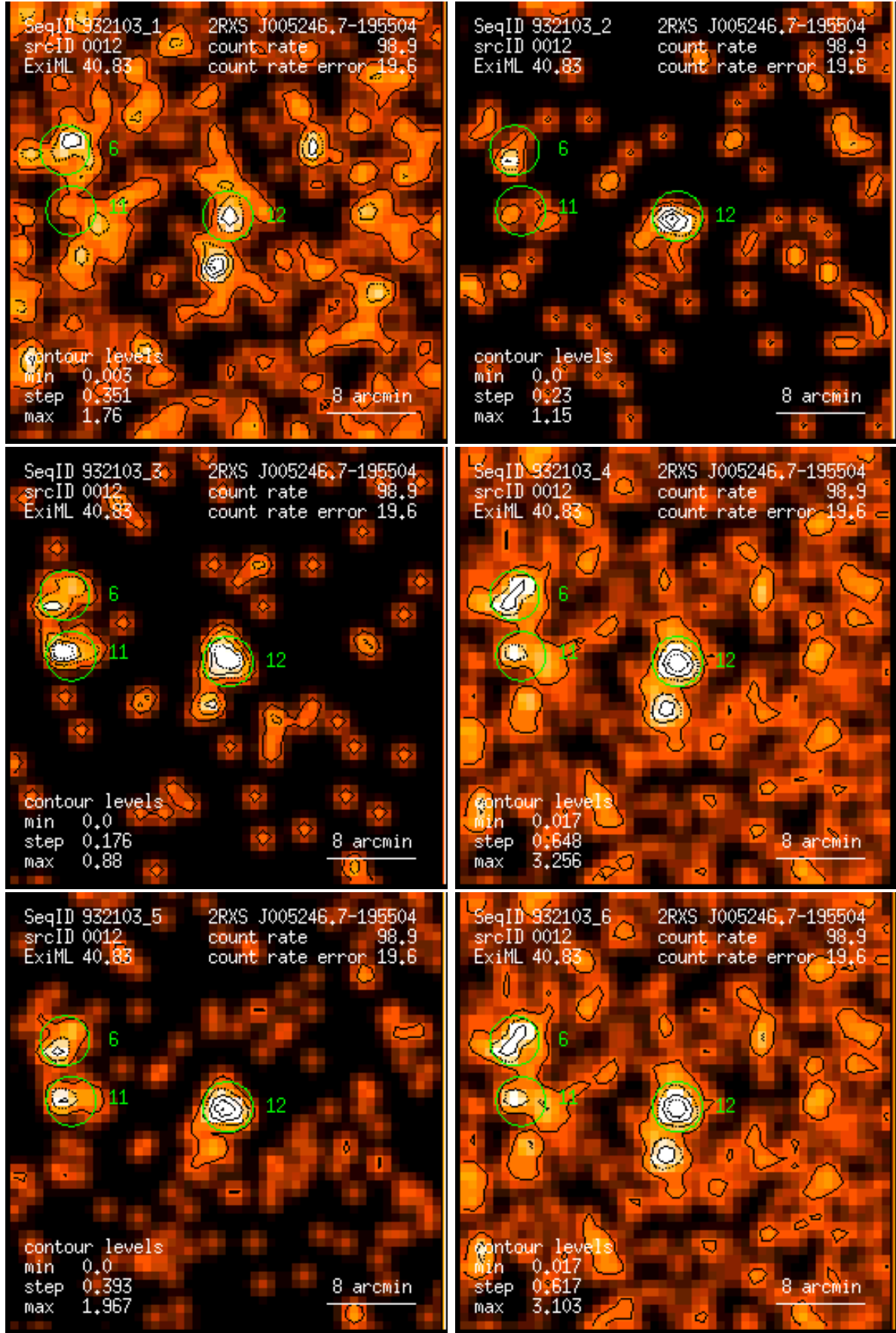
Figure 12: RASS 932103: detection 0012: band rate images, Gaussian filter: (1) PSPC channels 11 – 41, (2) 52 – 90, (3) 91 – 201, (4) 11 – 235, (5) 52 – 201, (6) 11 – 201. Broad band rates in counts/ks. Band rate contour levels in counts/ks/arcmin 2 .
