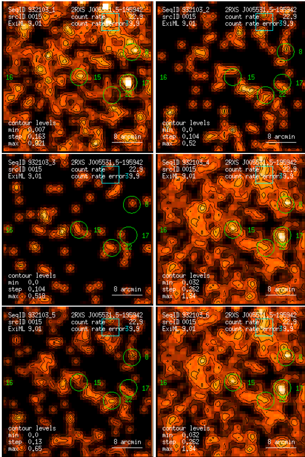
Figure 15: RASS 932103: detection 0015: band rate images, Gaussian filter: (1) PSPC channels 11 – 41, (2) 52 – 90, (3) 91 – 201, (4) 11 – 235, (5) 52 – 201, (6) 11 – 201. Broad band rates in counts/ks. Band rate contour levels in counts/ks/arcmin 2 .
