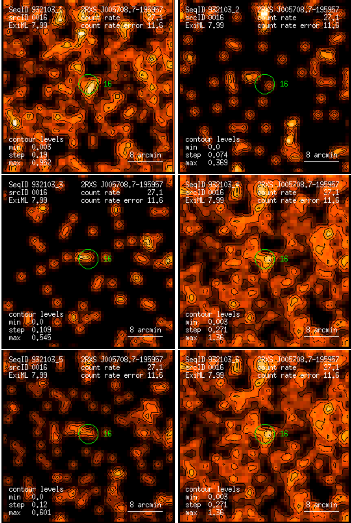
Figure 16: RASS 932103: detection 0016: band rate images, Gaussian filter: (1) PSPC channels 11 – 41, (2) 52 – 90, (3) 91 – 201, (4) 11 – 235, (5) 52 – 201, (6) 11 – 201. Broad band rates in counts/ks. Band rate contour levels in counts/ks/arcmin 2 .
