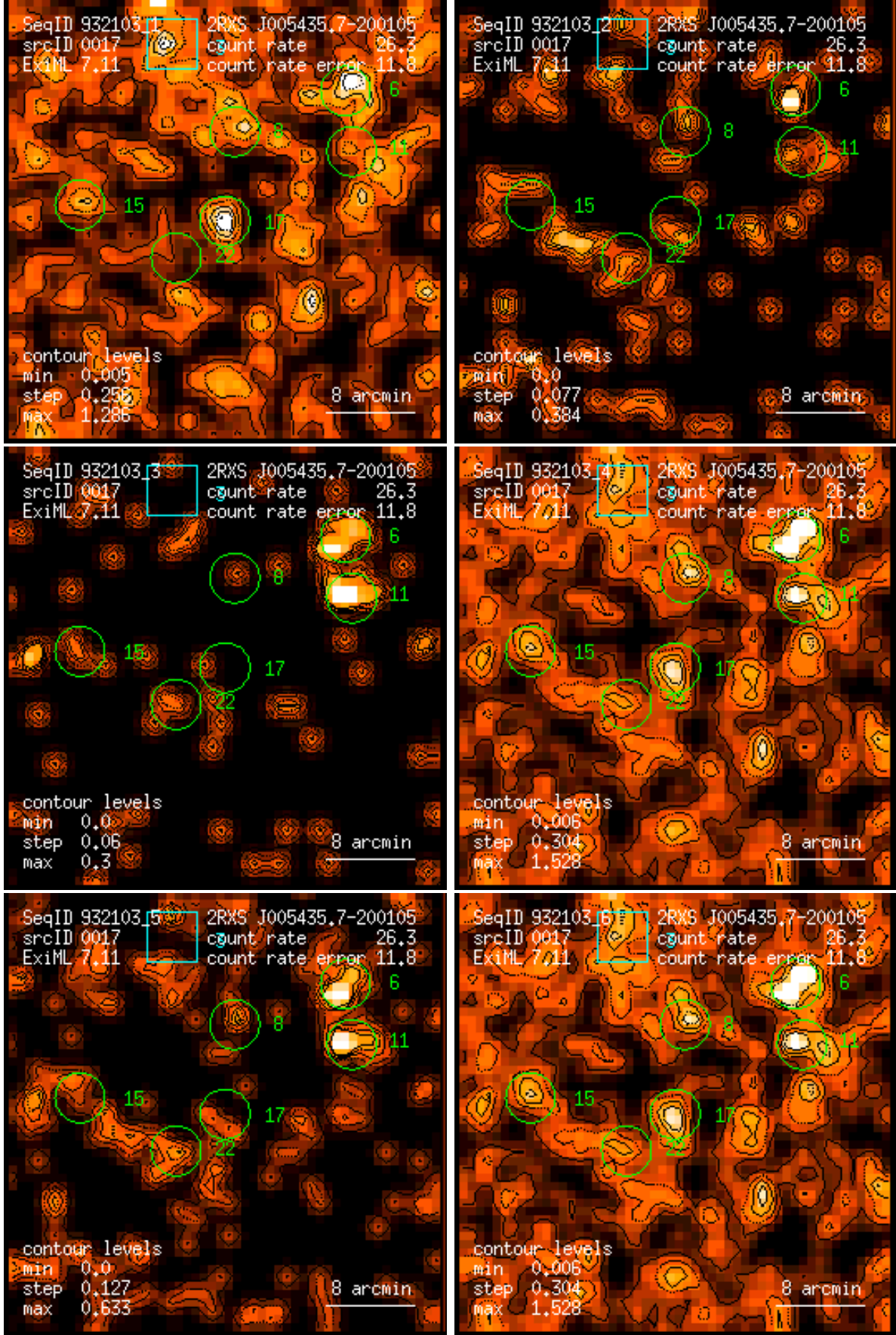
Figure 17: RASS 932103: detection 0017: band rate images, Gaussian filter: (1) PSPC channels 11 – 41, (2) 52 – 90, (3) 91 – 201, (4) 11 – 235, (5) 52 – 201, (6) 11 – 201. Broad band rates in counts/ks. Band rate contour levels in counts/ks/arcmin 2 .
