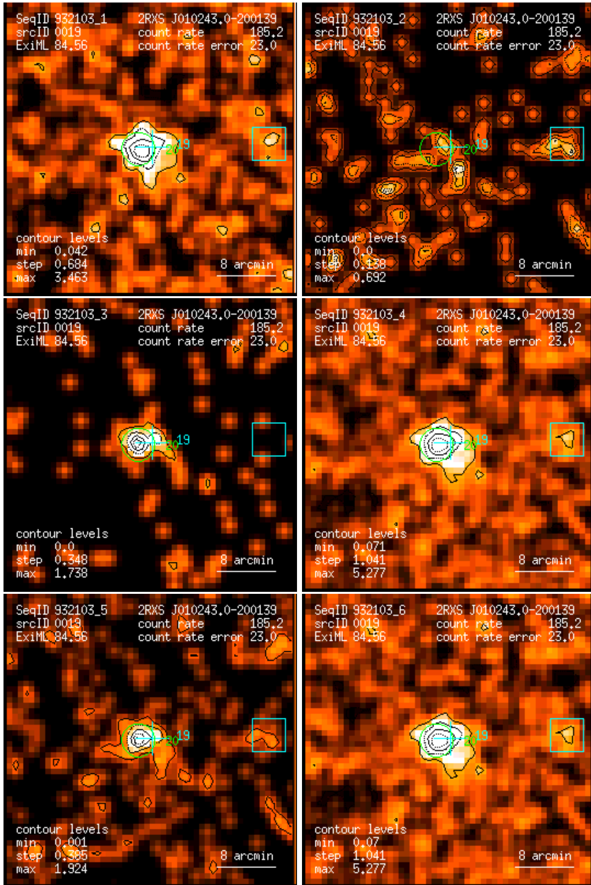
Figure 19: RASS 932103: detection 0019: band rate images, Gaussian filter: (1) PSPC channels 11 – 41, (2) 52 – 90, (3) 91 – 201, (4) 11 – 235, (5) 52 – 201, (6) 11 – 201. Broad band rates in counts/ks. Band rate contour levels in counts/ks/arcmin 2 .
