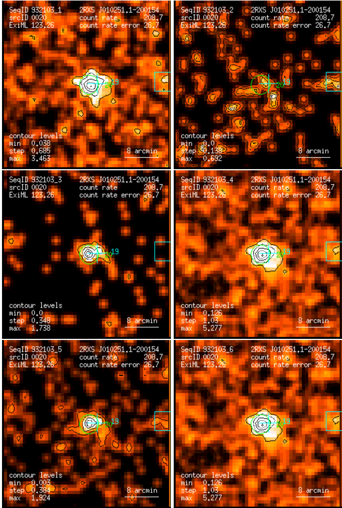
Figure 20: RASS 932103: detection 0020: band rate images, Gaussian filter: (1) PSPC channels 11 – 41, (2) 52 – 90, (3) 91 – 201, (4) 11 – 235, (5) 52 – 201, (6) 11 – 201. Broad band rates in counts/ks. Band rate contour levels in counts/ks/arcmin 2 .
