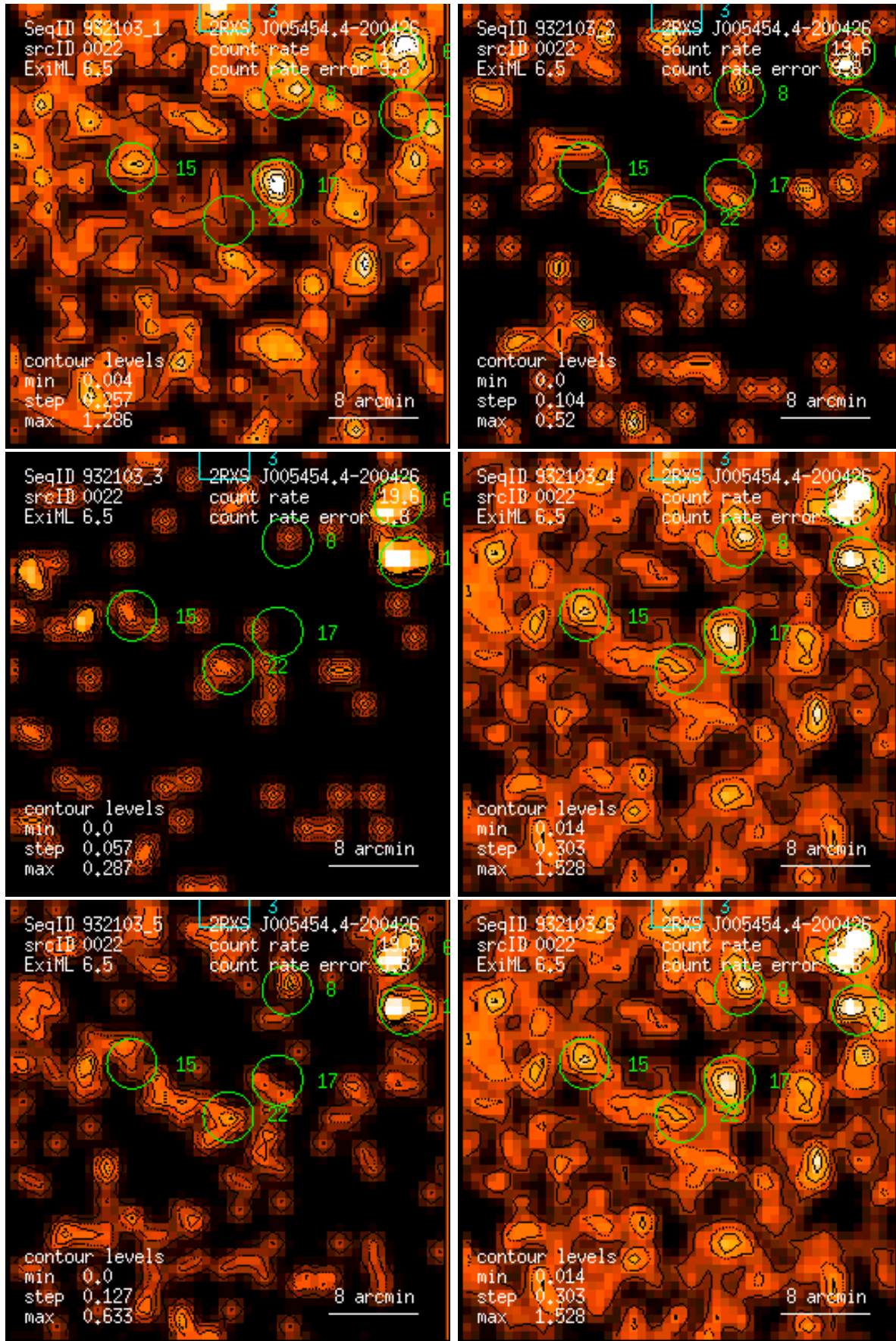
Figure 22: RASS 932103: detection 0022: band rate images, Gaussian filter: (1) PSPC channels 11 – 41, (2) 52 – 90, (3) 91 – 201, (4) 11 – 235, (5) 52 – 201, (6) 11 – 201. Broad band rates in counts/ks. Band rate contour levels in counts/ks/arcmin 2 .
