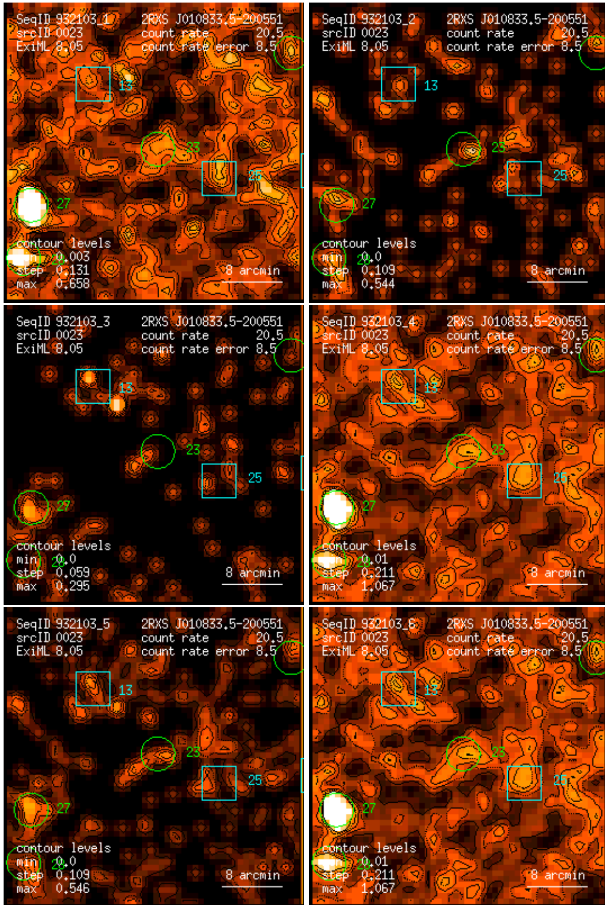
Figure 23: RASS 932103: detection 0023: band rate images, Gaussian filter: (1) PSPC channels 11 – 41, (2) 52 – 90, (3) 91 – 201, (4) 11 – 235, (5) 52 – 201, (6) 11 – 201. Broad band rates in counts/ks. Band rate contour levels in counts/ks/arcmin 2 .
