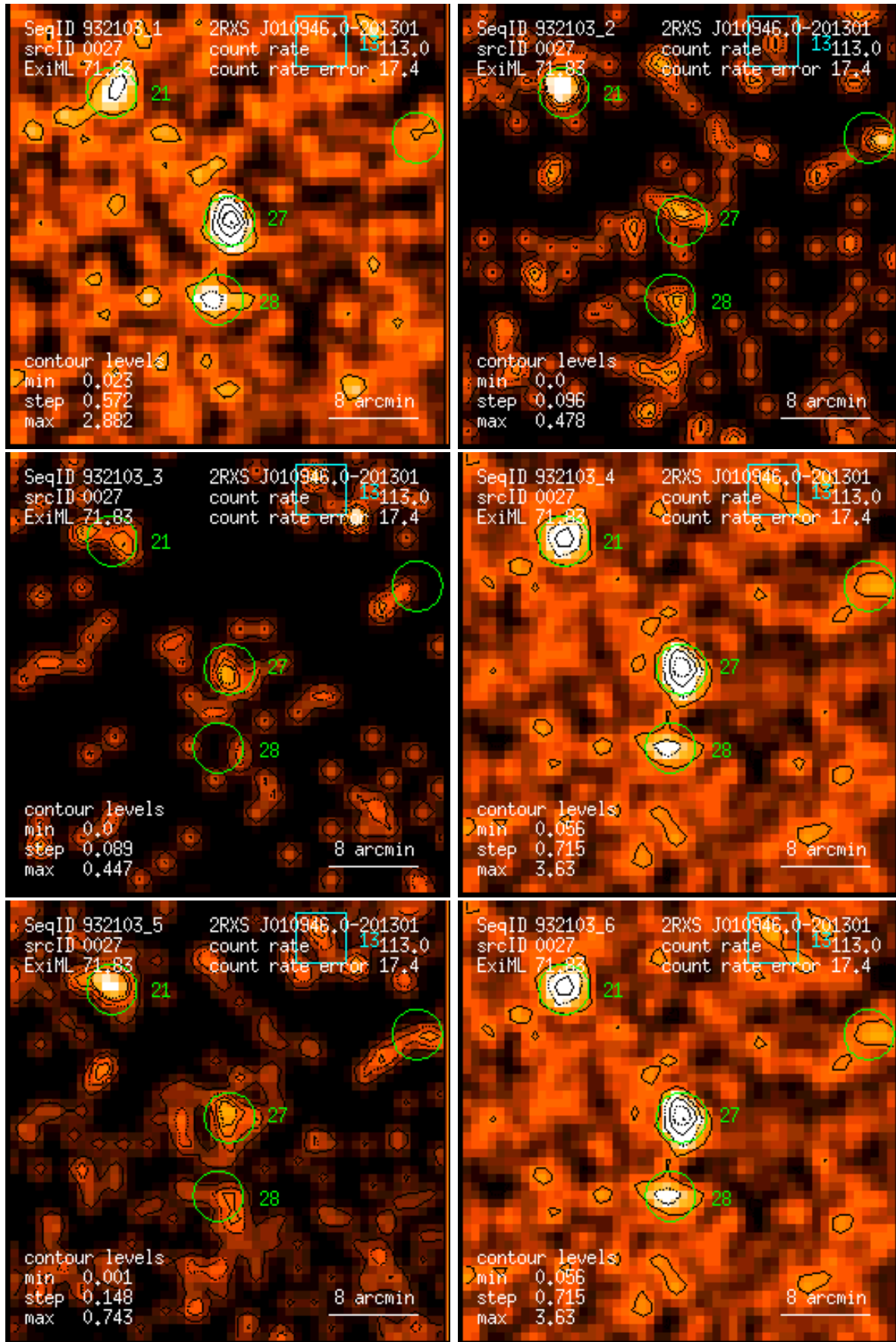
Figure 27: RASS 932103: detection 0027: band rate images, Gaussian filter: (1) PSPC channels 11 – 41, (2) 52 – 90, (3) 91 – 201, (4) 11 – 235, (5) 52 – 201, (6) 11 – 201. Broad band rates in counts/ks. Band rate contour levels in counts/ks/arcmin 2 .
